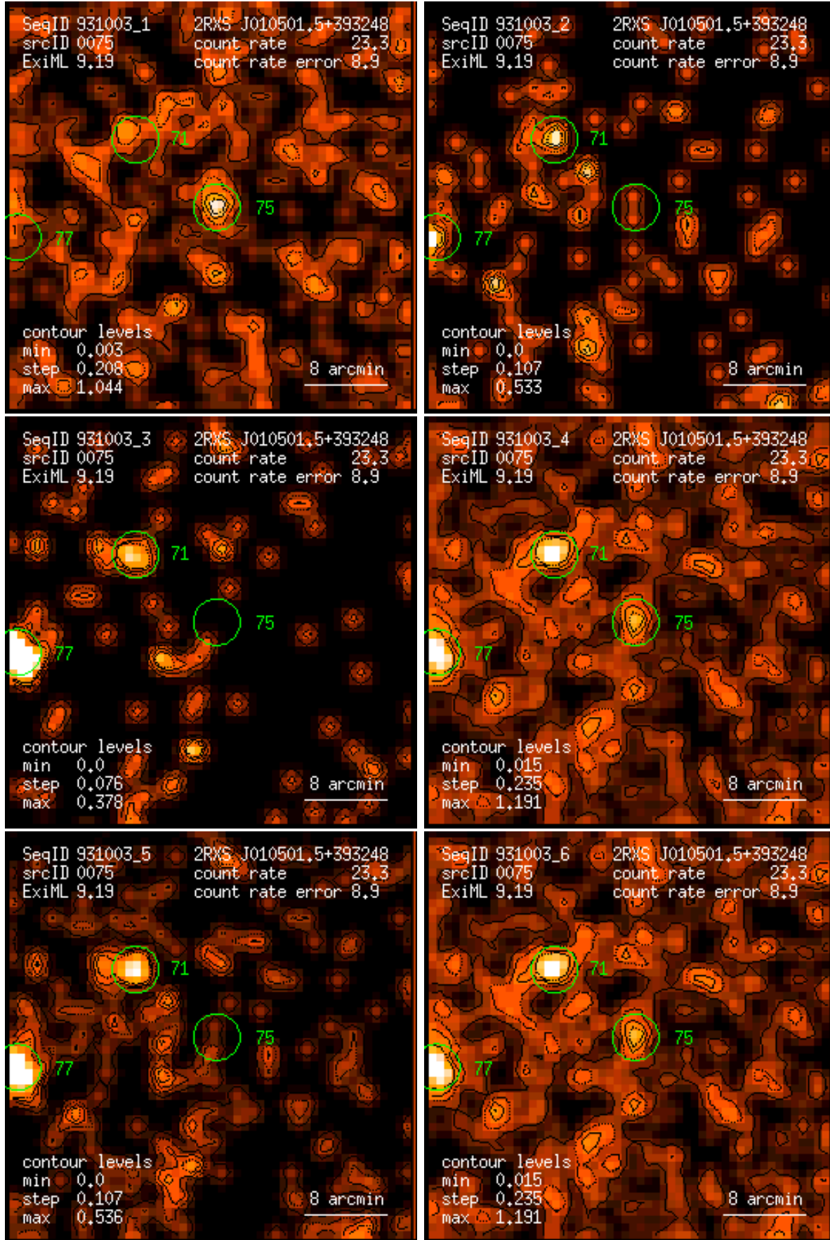
Figure 75: RASS 931003: detection 0075: band rate images, Gaussian filter: (1) PSPC channels 11 – 41, (2) 52 – 90, (3) 91 – 201, (4) 11 – 235, (5) 52 – 201, (6) 11 – 201. Broad band rates in counts/ks. Band rate contour levels in counts/ks/arcmin 2 .
