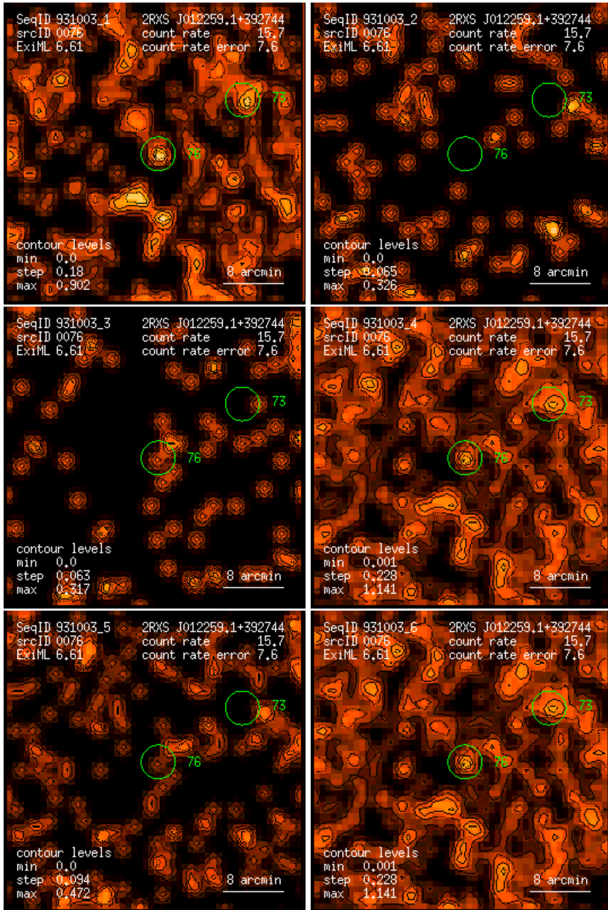
Figure 76: RASS 931003: detection 0076: band rate images, Gaussian filter: (1) PSPC channels 11 – 41, (2) 52 – 90, (3) 91 – 201, (4) 11 – 235, (5) 52 – 201, (6) 11 – 201. Broad band rates in counts/ks. Band rate contour levels in counts/ks/arcmin 2 .
