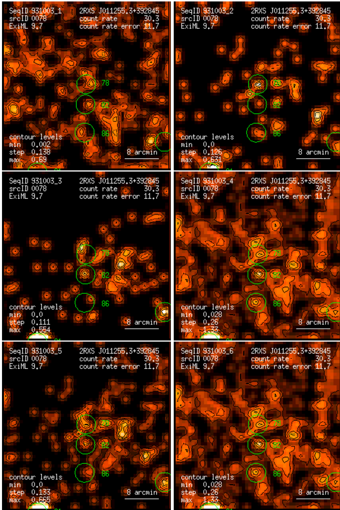
Figure 78: RASS 931003: detection 0078: band rate images, Gaussian filter: (1) PSPC channels 11 – 41, (2) 52 – 90, (3) 91 – 201, (4) 11 – 235, (5) 52 – 201, (6) 11 – 201. Broad band rates in counts/ks. Band rate contour levels in counts/ks/arcmin 2 .
