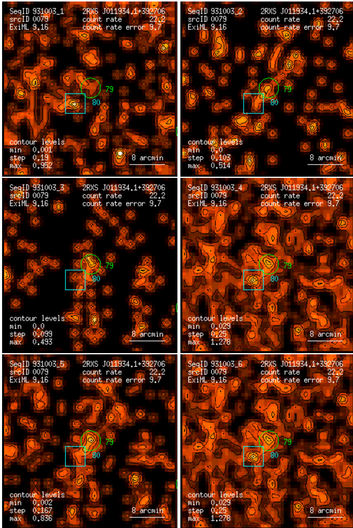
Figure 79: RASS 931003: detection 0079: band rate images, Gaussian filter: (1) PSPC channels 11 – 41, (2) 52 – 90, (3) 91 – 201, (4) 11 – 235, (5) 52 – 201, (6) 11 – 201. Broad band rates in counts/ks. Band rate contour levels in counts/ks/arcmin 2 .
