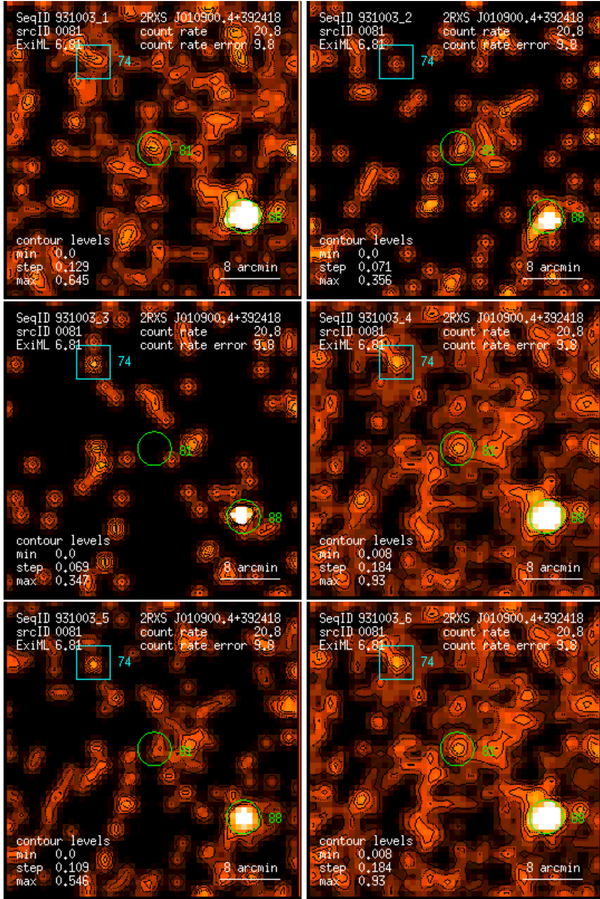
Figure 81: RASS 931003: detection 0081: band rate images, Gaussian filter: (1) PSPC channels 11 – 41, (2) 52 – 90, (3) 91 – 201, (4) 11 – 235, (5) 52 – 201, (6) 11 – 201. Broad band rates in counts/ks. Band rate contour levels in counts/ks/arcmin 2 .
