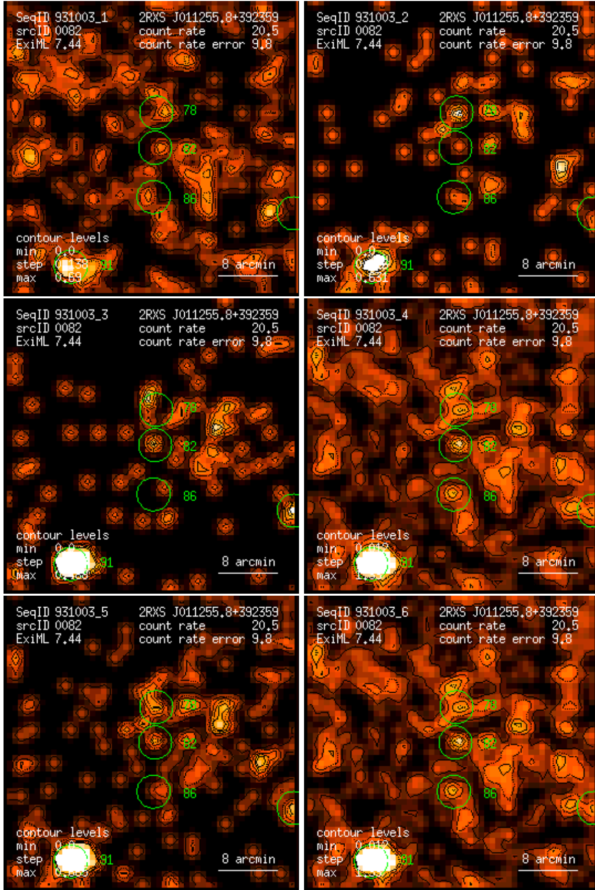
Figure 82: RASS 931003: detection 0082: band rate images, Gaussian filter: (1) PSPC channels 11 – 41, (2) 52 – 90, (3) 91 – 201, (4) 11 – 235, (5) 52 – 201, (6) 11 – 201. Broad band rates in counts/ks. Band rate contour levels in counts/ks/arcmin 2 .
