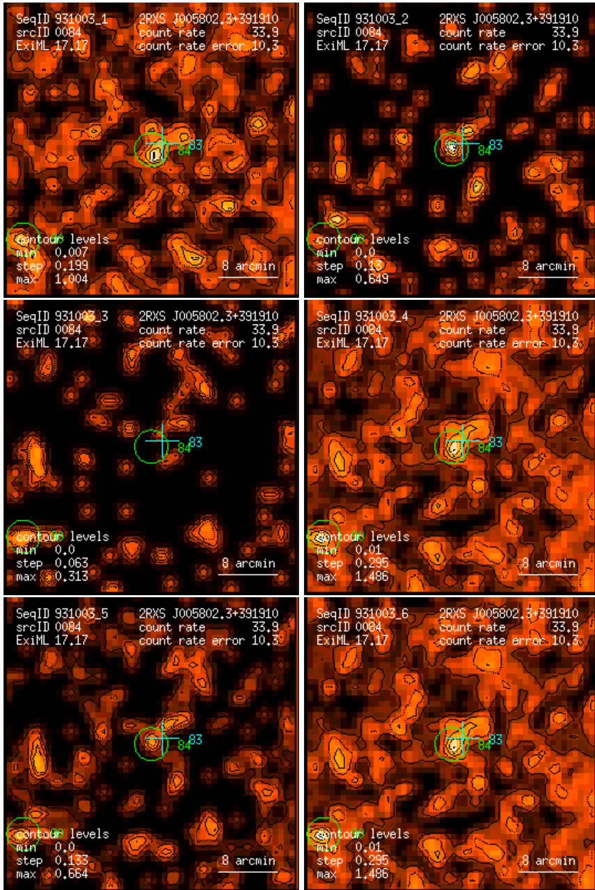
Figure 84: RASS 931003: detection 0084: band rate images, Gaussian filter: (1) PSPC channels 11 – 41, (2) 52 – 90, (3) 91 – 201, (4) 11 – 235, (5) 52 – 201, (6) 11 – 201. Broad band rates in counts/ks. Band rate contour levels in counts/ks/arcmin 2 .
