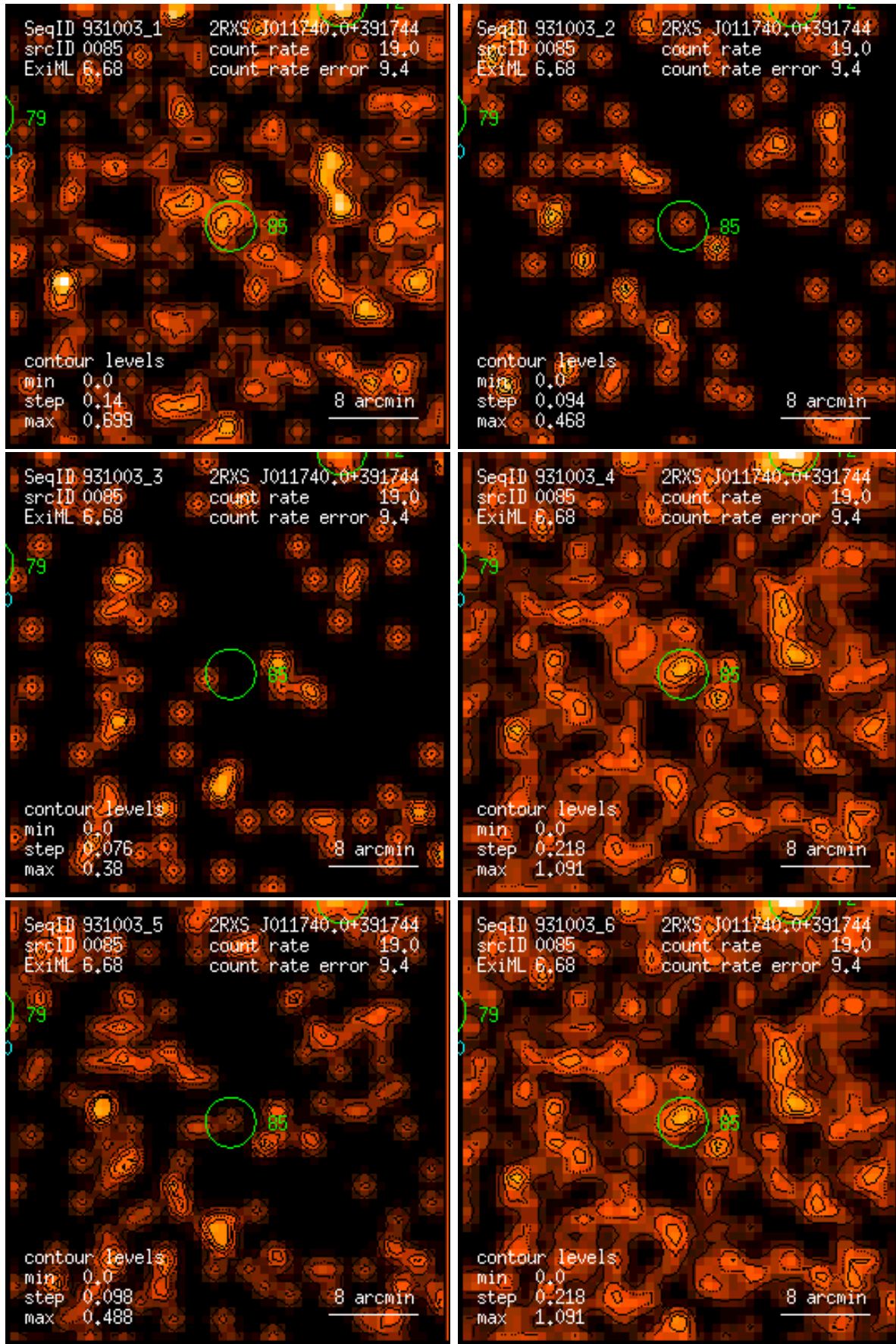
Figure 85: RASS 931003: detection 0085: band rate images, Gaussian filter: (1) PSPC channels 11 – 41, (2) 52 – 90, (3) 91 – 201, (4) 11 – 235, (5) 52 – 201, (6) 11 – 201. Broad band rates in counts/ks. Band rate contour levels in counts/ks/arcmin 2 .
