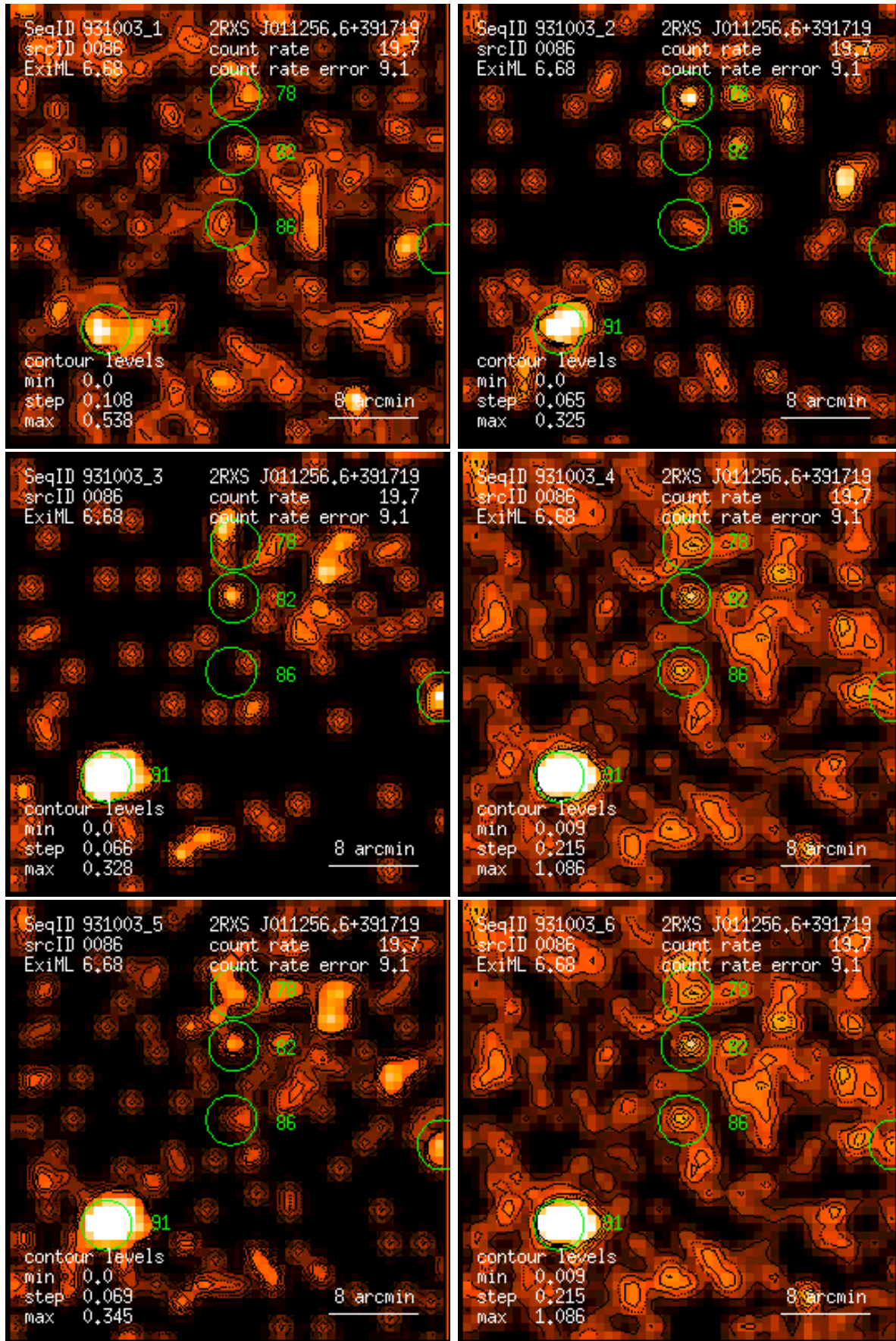
Figure 86: RASS 931003: detection 0086: band rate images, Gaussian filter: (1) PSPC channels 11 – 41, (2) 52 – 90, (3) 91 – 201, (4) 11 – 235, (5) 52 – 201, (6) 11 – 201. Broad band rates in counts/ks. Band rate contour levels in counts/ks/arcmin 2 .
