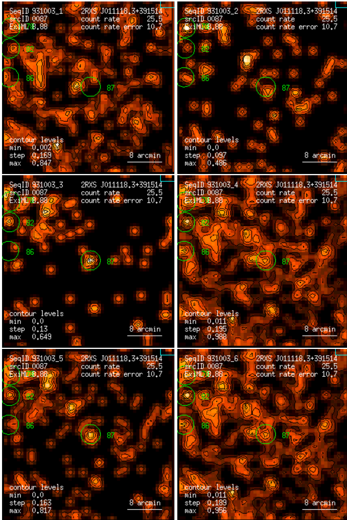
Figure 87: RASS 931003: detection 0087: band rate images, Gaussian filter: (1) PSPC channels 11 – 41, (2) 52 – 90, (3) 91 – 201, (4) 11 – 235, (5) 52 – 201, (6) 11 – 201. Broad band rates in counts/ks. Band rate contour levels in counts/ks/arcmin 2 .
