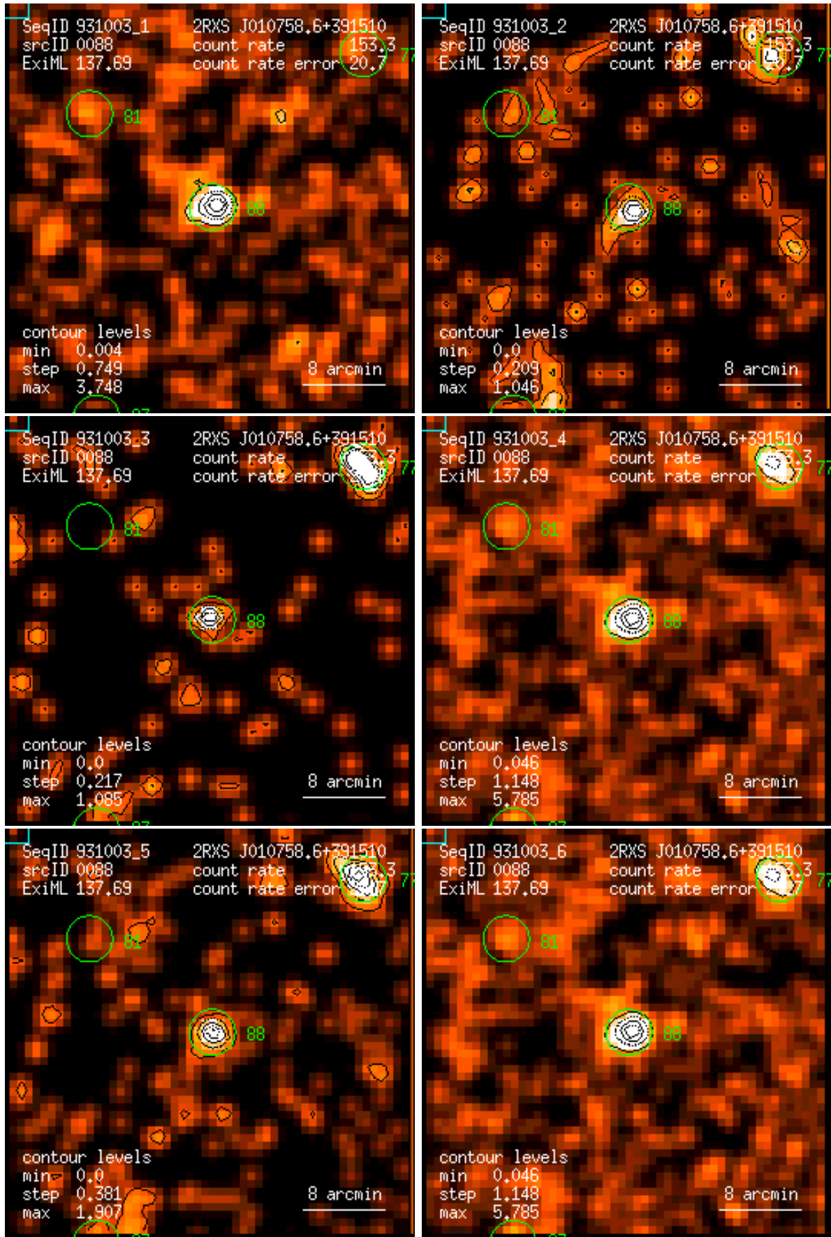
Figure 88: RASS 931003: detection 0088: band rate images, Gaussian filter: (1) PSPC channels 11 – 41, (2) 52 – 90, (3) 91 – 201, (4) 11 – 235, (5) 52 – 201, (6) 11 – 201. Broad band rates in counts/ks. Band rate contour levels in counts/ks/arcmin 2 .
