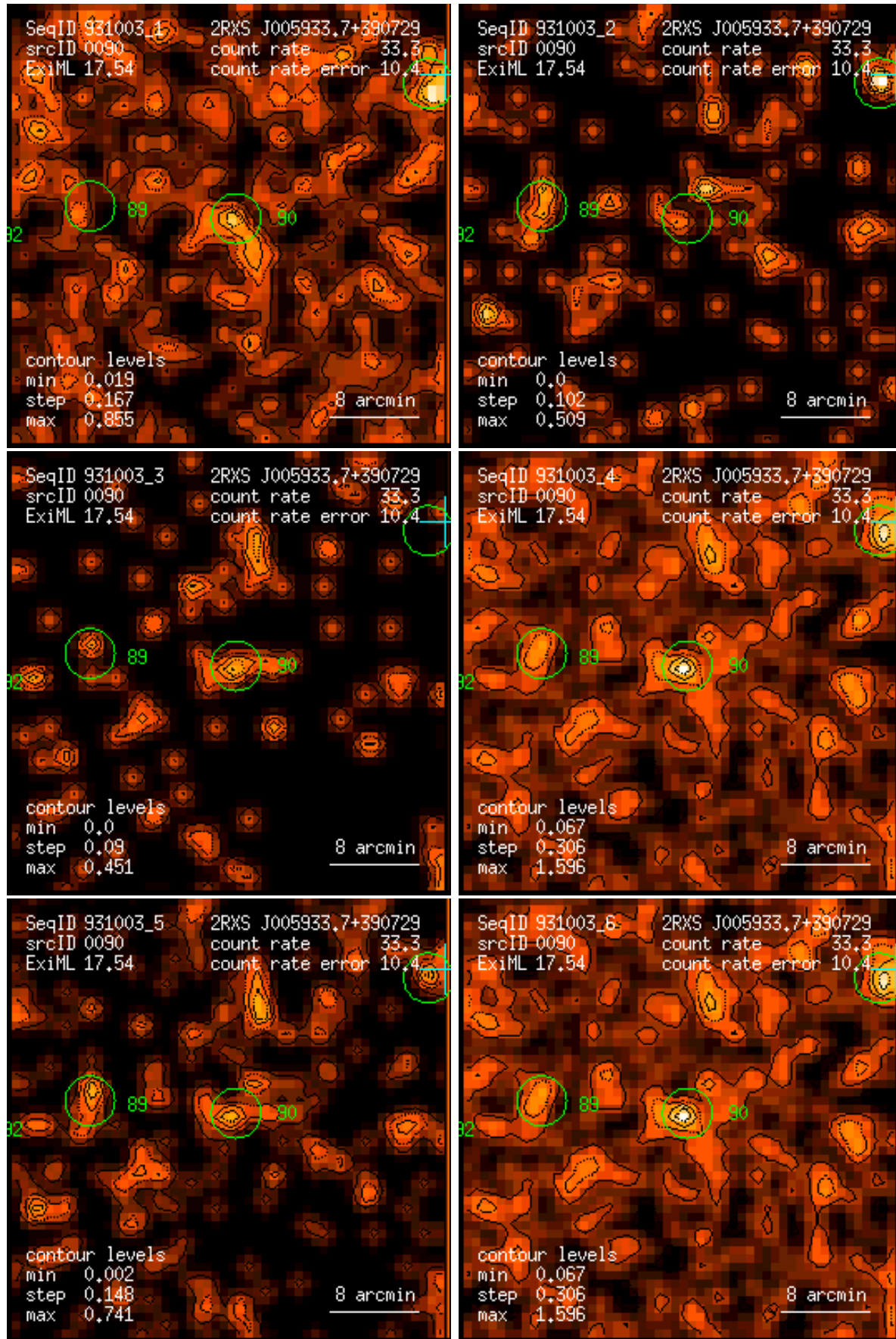
Figure 90: RASS 931003: detection 0090: band rate images, Gaussian filter: (1) PSPC channels 11 – 41, (2) 52 – 90, (3) 91 – 201, (4) 11 – 235, (5) 52 – 201, (6) 11 – 201. Broad band rates in counts/ks. Band rate contour levels in counts/ks/arcmin 2 .
