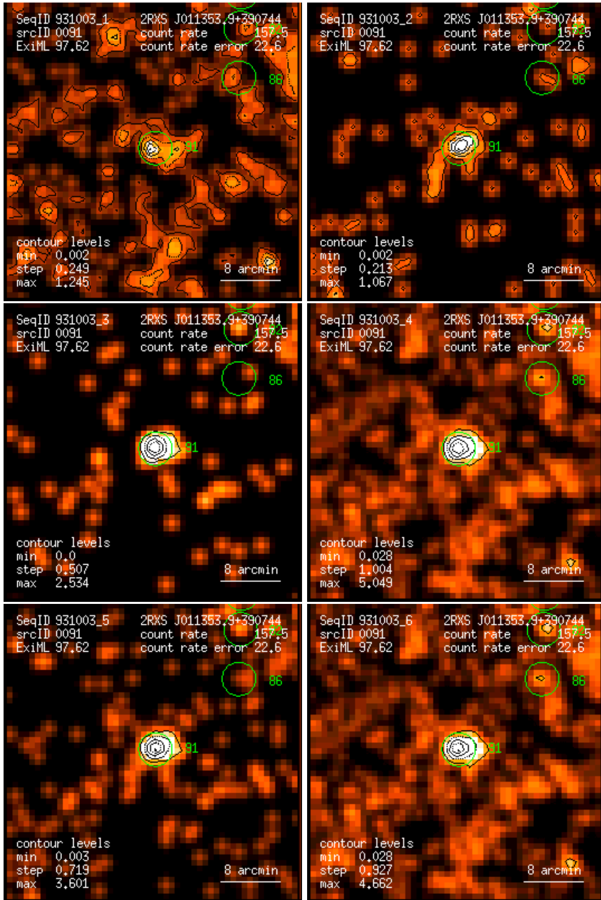
Figure 91: RASS 931003: detection 0091: band rate images, Gaussian filter: (1) PSPC channels 11 – 41, (2) 52 – 90, (3) 91 – 201, (4) 11 – 235, (5) 52 – 201, (6) 11 – 201. Broad band rates in counts/ks. Band rate contour levels in counts/ks/arcmin 2 .
