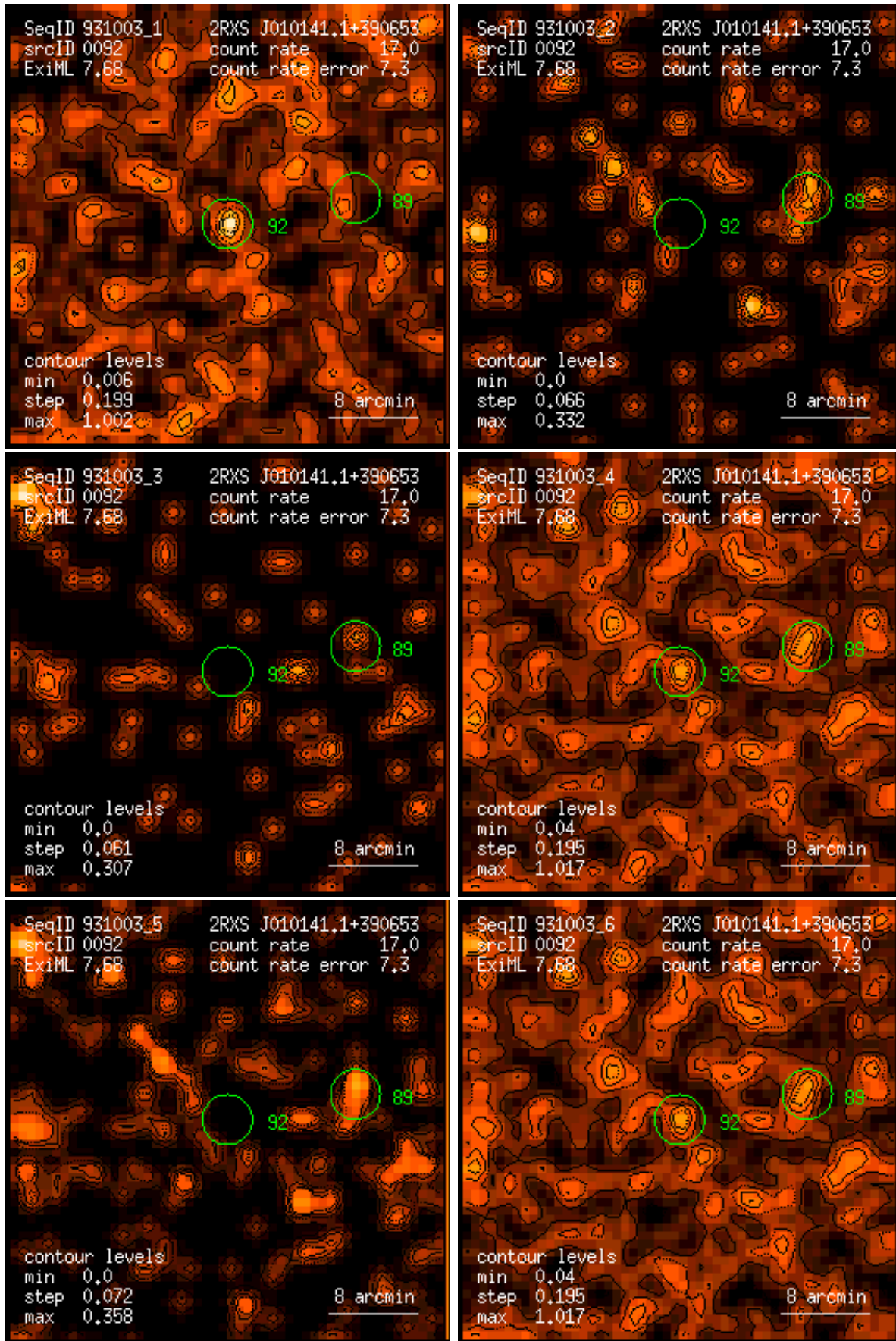
Figure 92: RASS 931003: detection 0092: band rate images, Gaussian filter: (1) PSPC channels 11 – 41, (2) 52 – 90, (3) 91 – 201, (4) 11 – 235, (5) 52 – 201, (6) 11 – 201. Broad band rates in counts/ks. Band rate contour levels in counts/ks/arcmin 2 .
