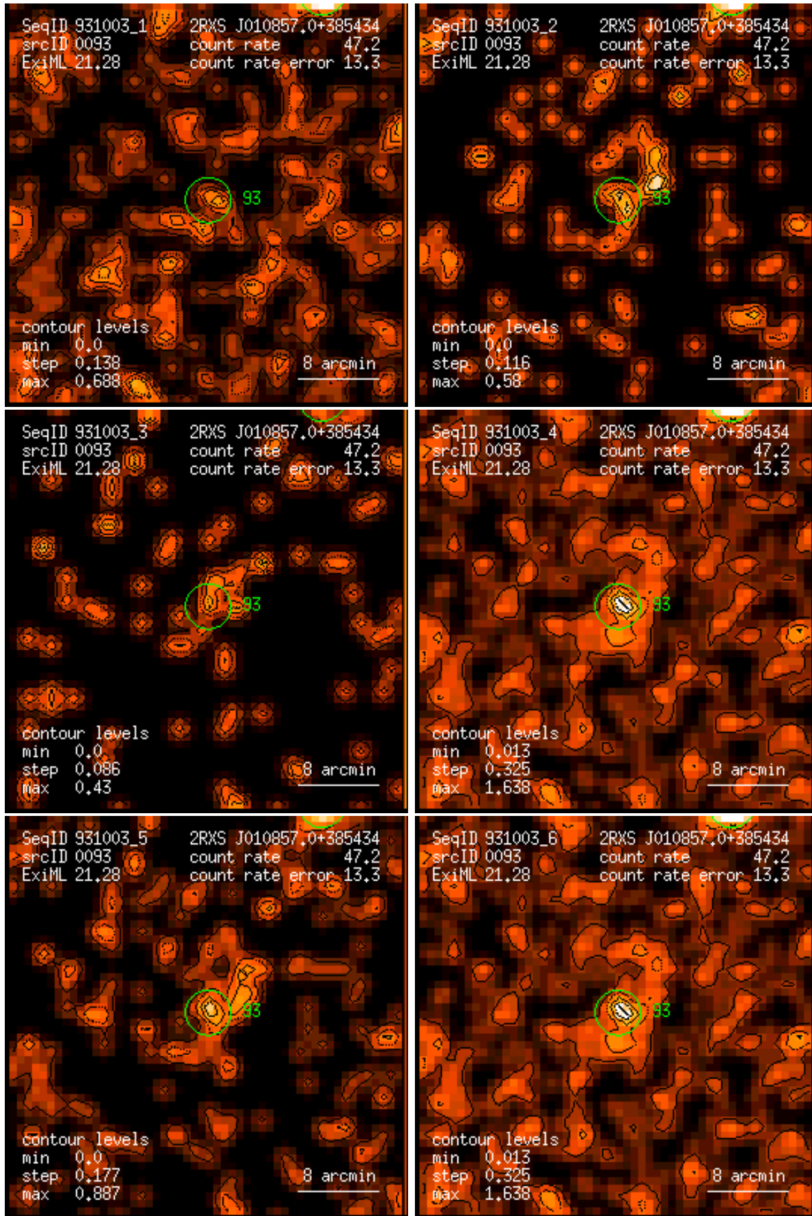
Figure 93: RASS 931003: detection 0093: band rate images, Gaussian filter: (1) PSPC channels 11 – 41, (2) 52 – 90, (3) 91 – 201, (4) 11 – 235, (5) 52 – 201, (6) 11 – 201. Broad band rates in counts/ks. Band rate contour levels in counts/ks/arcmin 2 .
