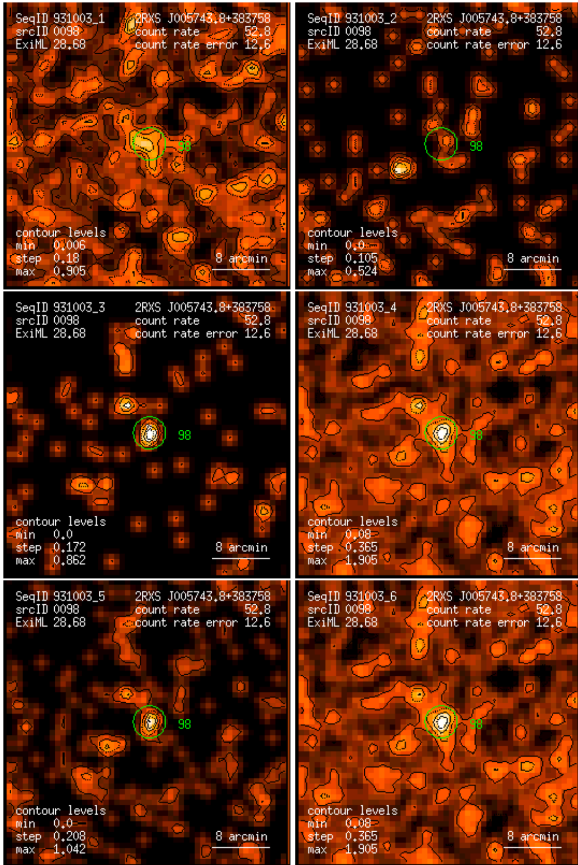
Figure 98: RASS 931003: detection 0098: band rate images, Gaussian filter: (1) PSPC channels 11 – 41, (2) 52 – 90, (3) 91 – 201, (4) 11 – 235, (5) 52 – 201, (6) 11 – 201. Broad band rates in counts/ks. Band rate contour levels in counts/ks/arcmin 2 .
