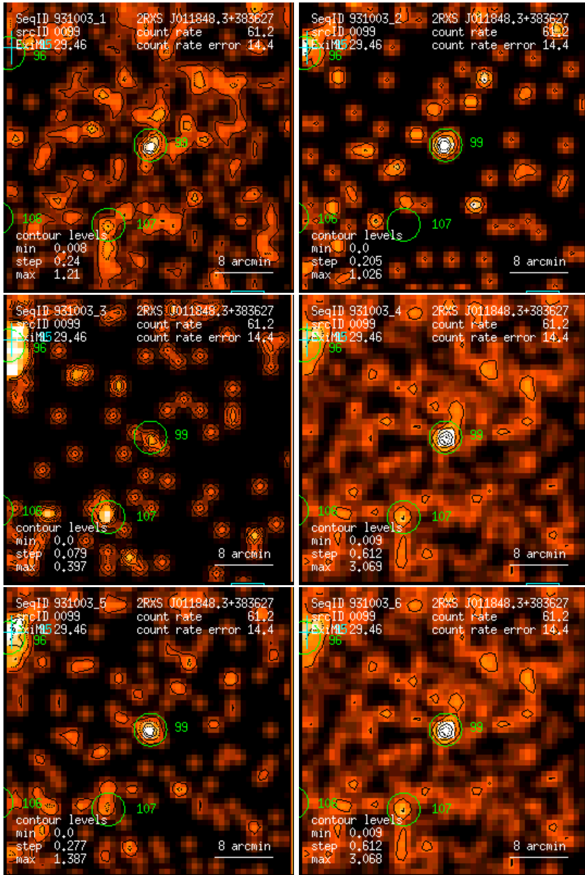
Figure 99: RASS 931003: detection 0099: band rate images, Gaussian filter: (1) PSPC channels 11 – 41, (2) 52 – 90, (3) 91 – 201, (4) 11 – 235, (5) 52 – 201, (6) 11 – 201. Broad band rates in counts/ks. Band rate contour levels in counts/ks/arcmin 2 .
