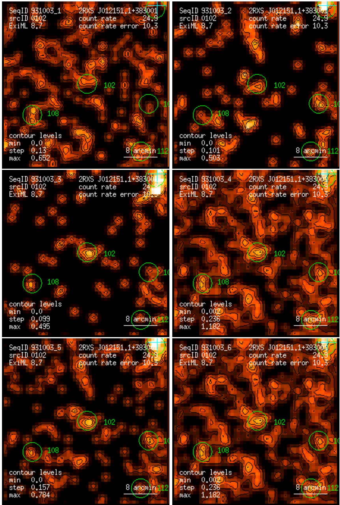
Figure 102: RASS 931003: detection 0102: band rate images, Gaussian filter: (1) PSPC channels 11 – 41, (2) 52 – 90, (3) 91 – 201, (4) 11 – 235, (5) 52 – 201, (6) 11 – 201. Broad band rates in counts/ks. Band rate contour levels in counts/ks/arcmin 2 .
