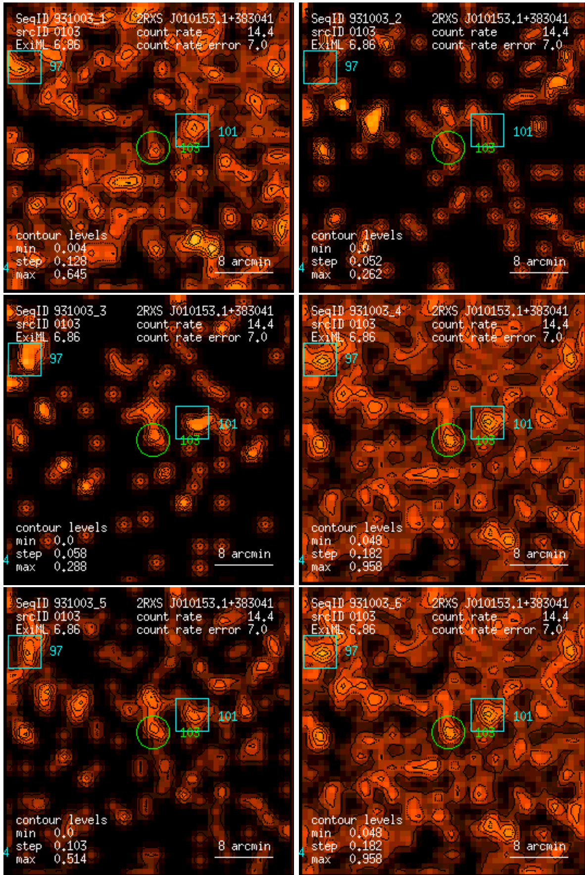
Figure 103: RASS 931003: detection 0103: band rate images, Gaussian filter: (1) PSPC channels 11 – 41, (2) 52 – 90, (3) 91 – 201, (4) 11 – 235, (5) 52 – 201, (6) 11 – 201. Broad band rates in counts/ks. Band rate contour levels in counts/ks/arcmin 2 .
