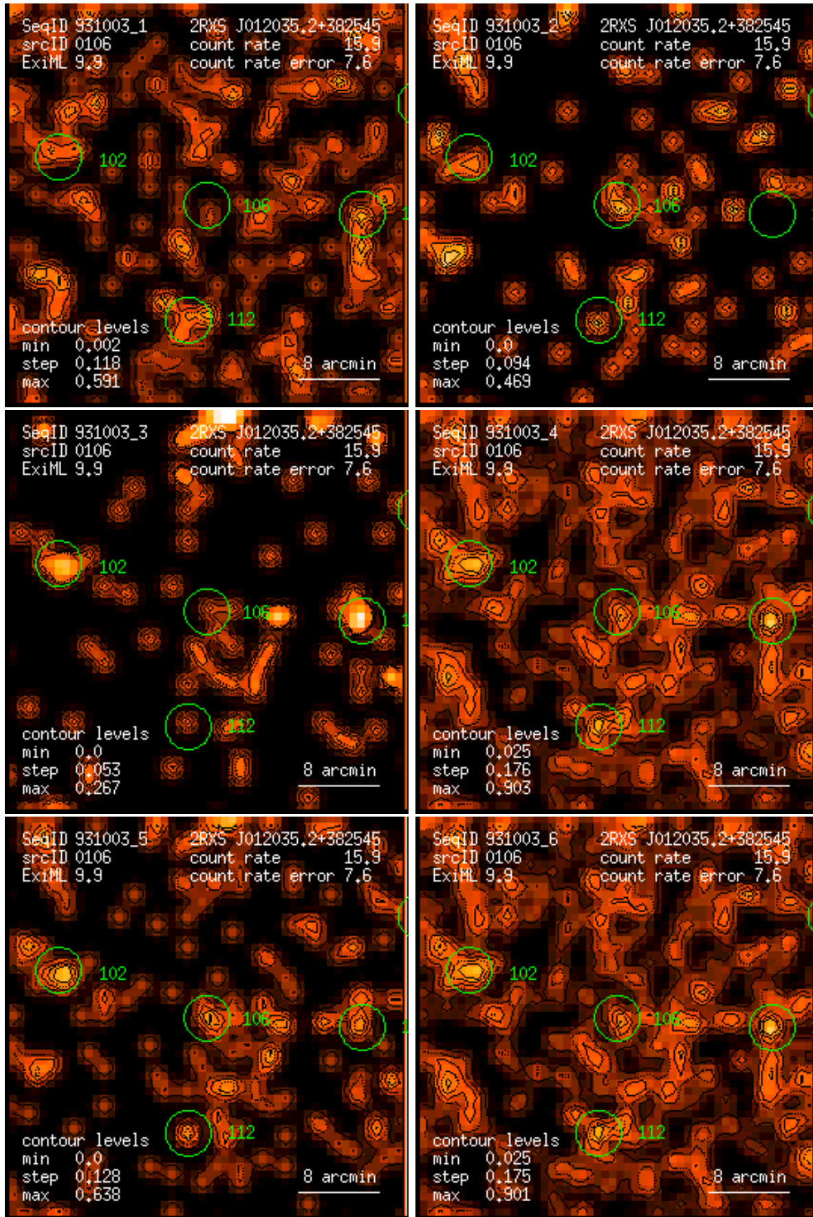
Figure 106: RASS 931003: detection 0106: band rate images, Gaussian filter: (1) PSPC channels 11 – 41, (2) 52 – 90, (3) 91 – 201, (4) 11 – 235, (5) 52 – 201, (6) 11 – 201. Broad band rates in counts/ks. Band rate contour levels in counts/ks/arcmin 2 .
