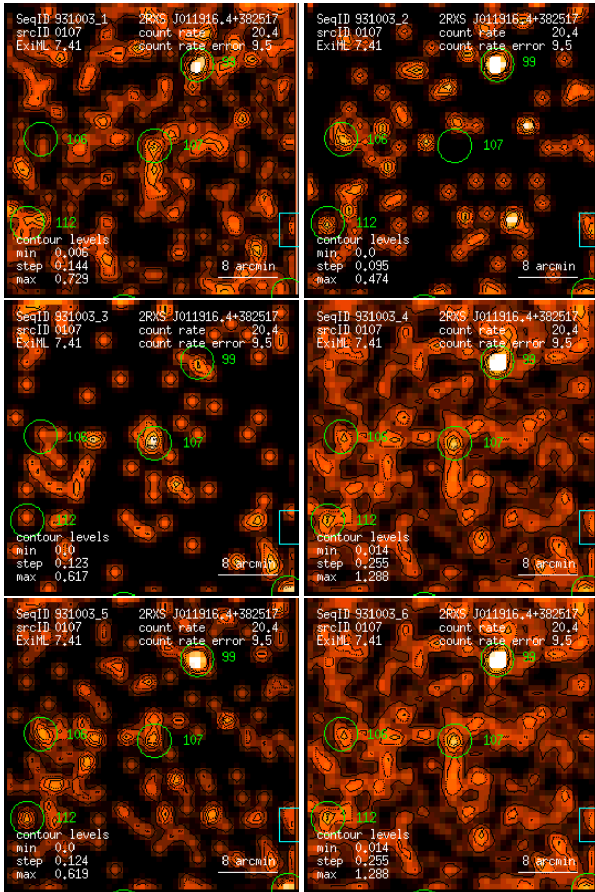
Figure 107: RASS 931003: detection 0107: band rate images, Gaussian filter: (1) PSPC channels 11 – 41, (2) 52 – 90, (3) 91 – 201, (4) 11 – 235, (5) 52 – 201, (6) 11 – 201. Broad band rates in counts/ks. Band rate contour levels in counts/ks/arcmin 2 .
