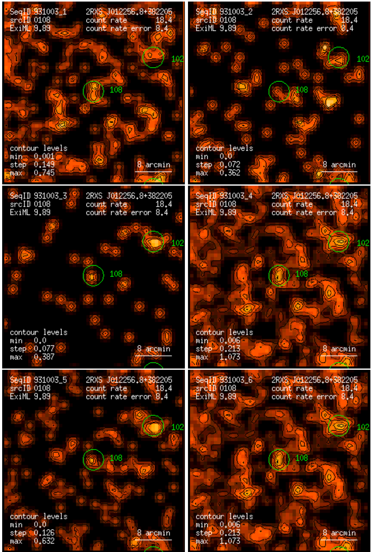
Figure 108: RASS 931003: detection 0108: band rate images, Gaussian filter: (1) PSPC channels 11 – 41, (2) 52 – 90, (3) 91 – 201, (4) 11 – 235, (5) 52 – 201, (6) 11 – 201. Broad band rates in counts/ks. Band rate contour levels in counts/ks/arcmin 2 .
