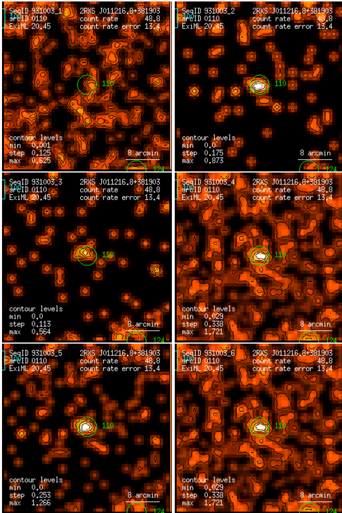
Figure 110: RASS 931003: detection 0110: band rate images, Gaussian filter: (1) PSPC channels 11 – 41, (2) 52 – 90, (3) 91 – 201, (4) 11 – 235, (5) 52 – 201, (6) 11 – 201. Broad band rates in counts/ks. Band rate contour levels in counts/ks/arcmin 2 .
