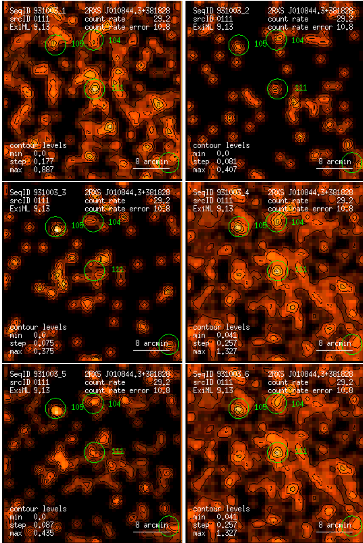
Figure 111: RASS 931003: detection 0111: band rate images, Gaussian filter: (1) PSPC channels 11 – 41, (2) 52 – 90, (3) 91 – 201, (4) 11 – 235, (5) 52 – 201, (6) 11 – 201. Broad band rates in counts/ks. Band rate contour levels in counts/ks/arcmin 2 .
