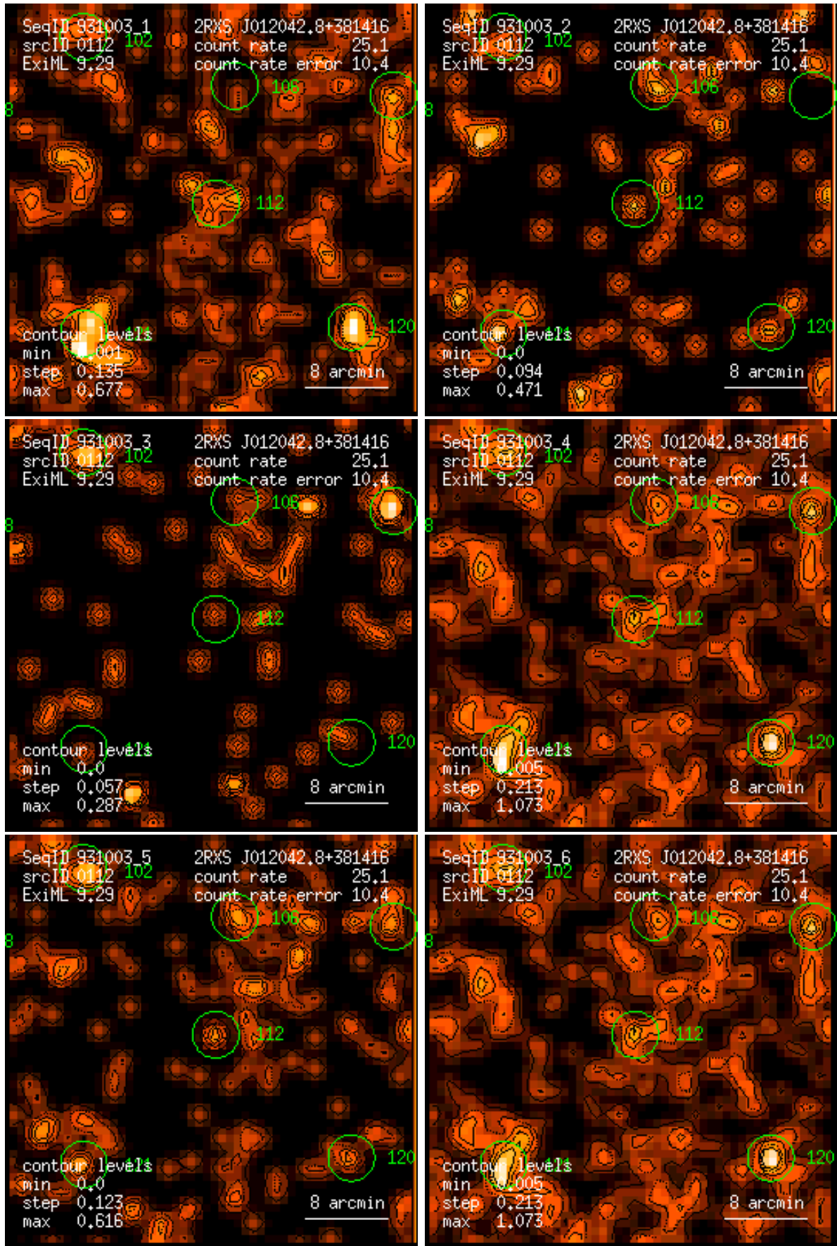
Figure 112: RASS 931003: detection 0112: band rate images, Gaussian filter: (1) PSPC channels 11 – 41, (2) 52 – 90, (3) 91 – 201, (4) 11 – 235, (5) 52 – 201, (6) 11 – 201. Broad band rates in counts/ks. Band rate contour levels in counts/ks/arcmin 2 .
