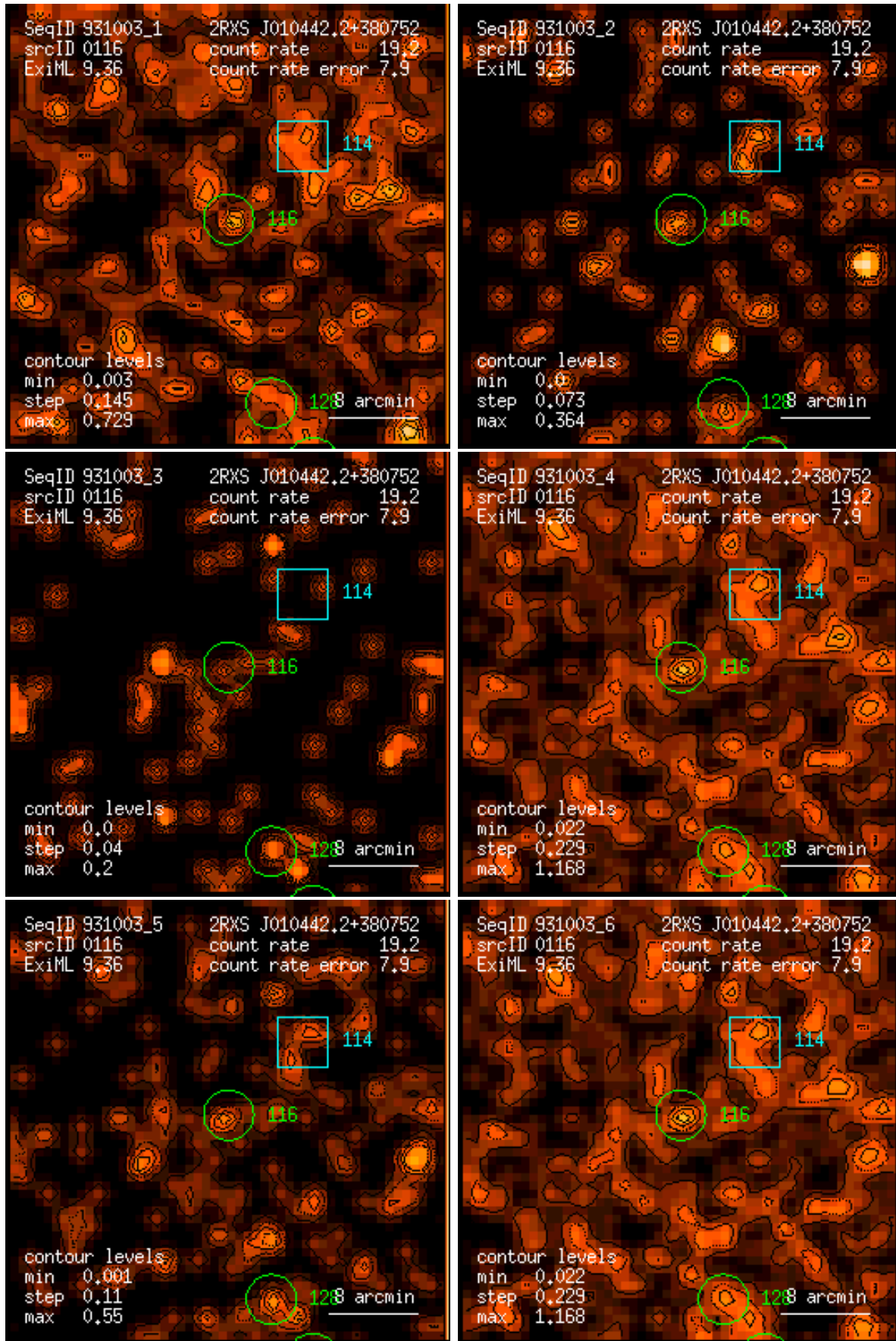
Figure 116: RASS 931003: detection 0116: band rate images, Gaussian filter: (1) PSPC channels 11 – 41, (2) 52 – 90, (3) 91 – 201, (4) 11 – 235, (5) 52 – 201, (6) 11 – 201. Broad band rates in counts/ks. Band rate contour levels in counts/ks/arcmin 2 .
