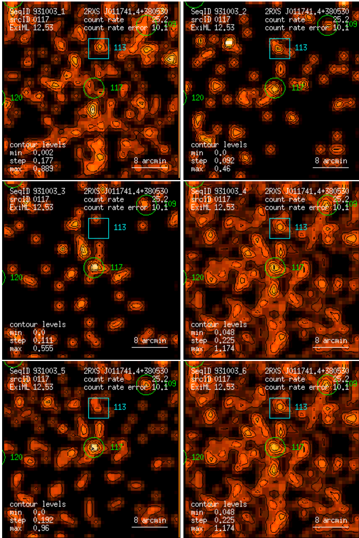
Figure 117: RASS 931003: detection 0117: band rate images, Gaussian filter: (1) PSPC channels 11 – 41, (2) 52 – 90, (3) 91 – 201, (4) 11 – 235, (5) 52 – 201, (6) 11 – 201. Broad band rates in counts/ks. Band rate contour levels in counts/ks/arcmin 2 .
