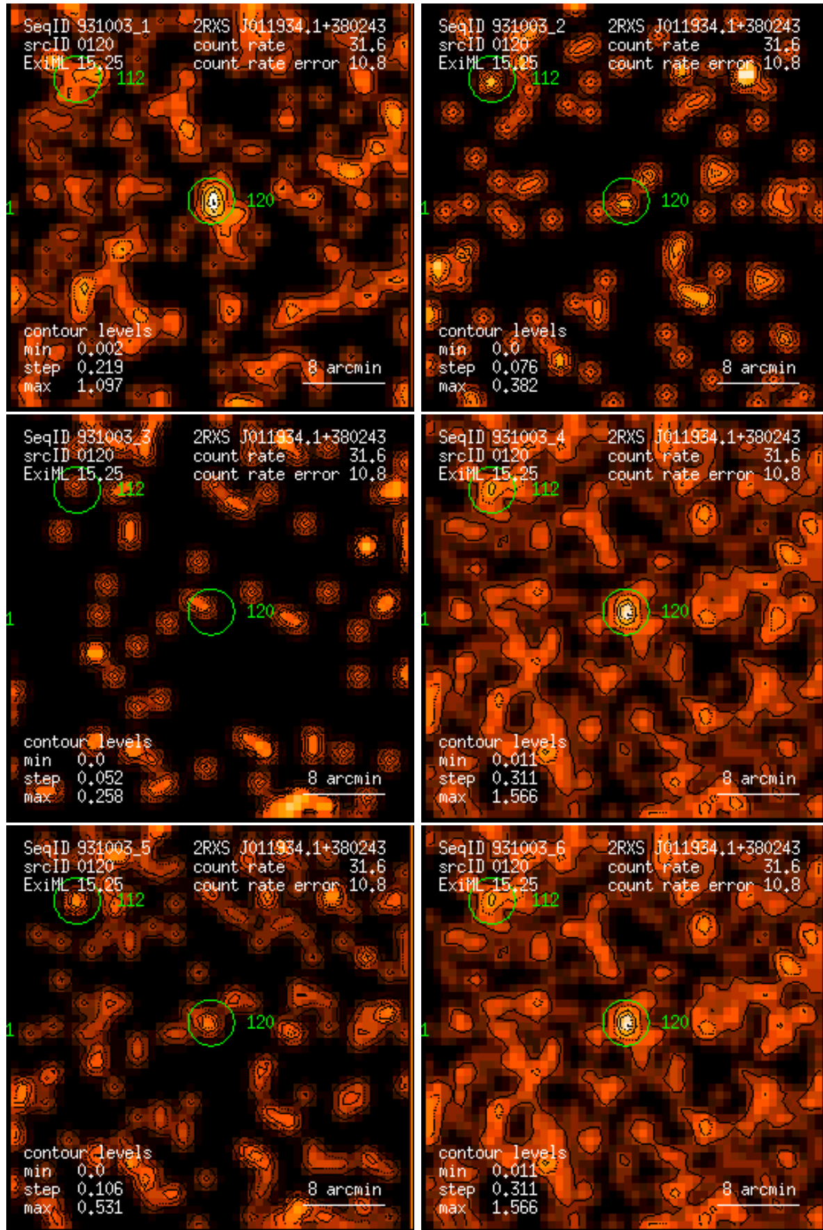
Figure 120: RASS 931003: detection 0120: band rate images, Gaussian filter: (1) PSPC channels 11 – 41, (2) 52 – 90, (3) 91 – 201, (4) 11 – 235, (5) 52 – 201, (6) 11 – 201. Broad band rates in counts/ks. Band rate contour levels in counts/ks/arcmin 2 .
