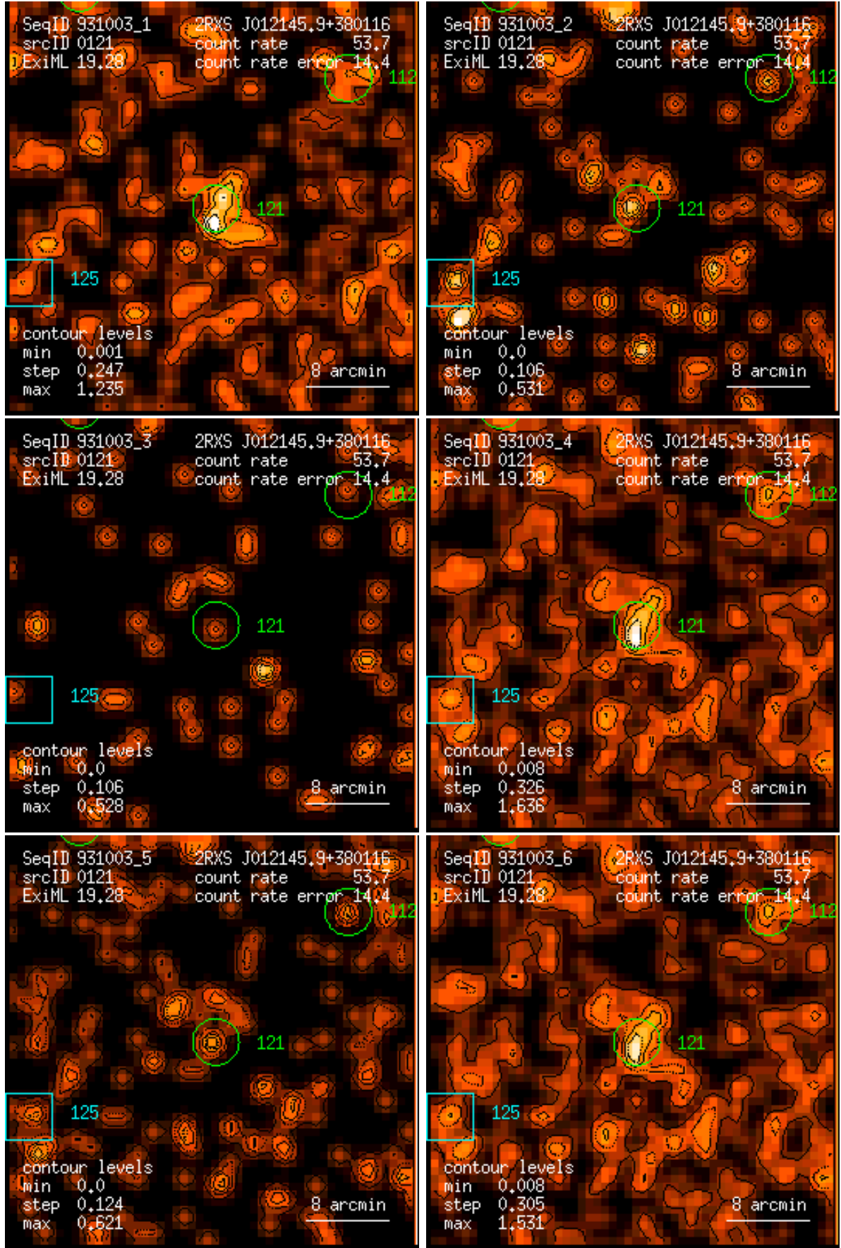
Figure 121: RASS 931003: detection 0121: band rate images, Gaussian filter: (1) PSPC channels 11 – 41, (2) 52 – 90, (3) 91 – 201, (4) 11 – 235, (5) 52 – 201, (6) 11 – 201. Broad band rates in counts/ks. Band rate contour levels in counts/ks/arcmin 2 .
