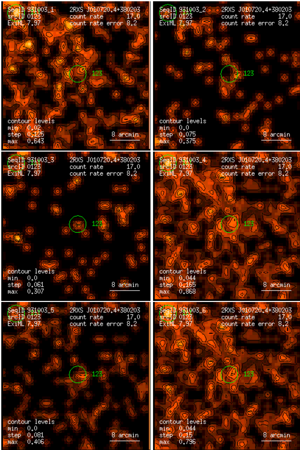
Figure 123: RASS 931003: detection 0123: band rate images, Gaussian filter: (1) PSPC channels 11 – 41, (2) 52 – 90, (3) 91 – 201, (4) 11 – 235, (5) 52 – 201, (6) 11 – 201. Broad band rates in counts/ks. Band rate contour levels in counts/ks/arcmin 2 .
