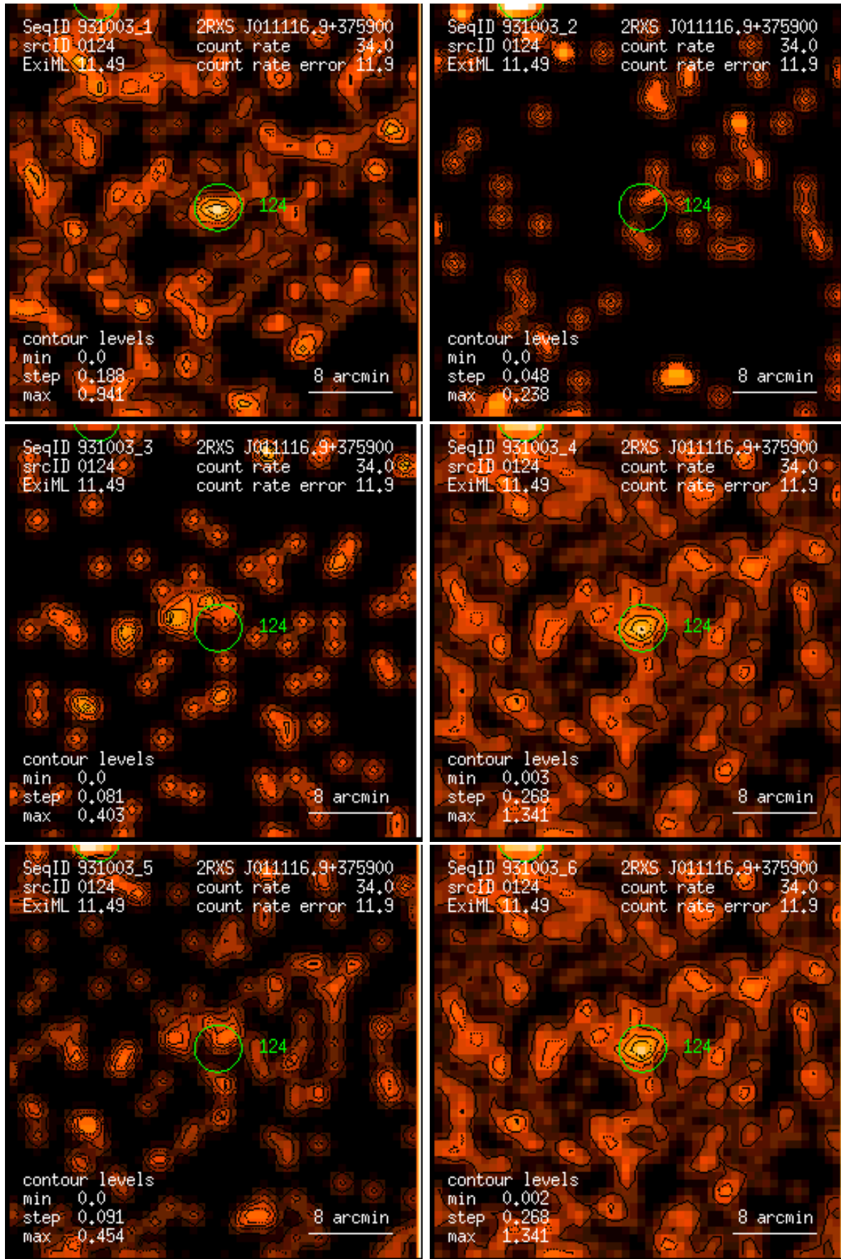
Figure 124: RASS 931003: detection 0124: band rate images, Gaussian filter: (1) PSPC channels 11 – 41, (2) 52 – 90, (3) 91 – 201, (4) 11 – 235, (5) 52 – 201, (6) 11 – 201. Broad band rates in counts/ks. Band rate contour levels in counts/ks/arcmin 2 .
