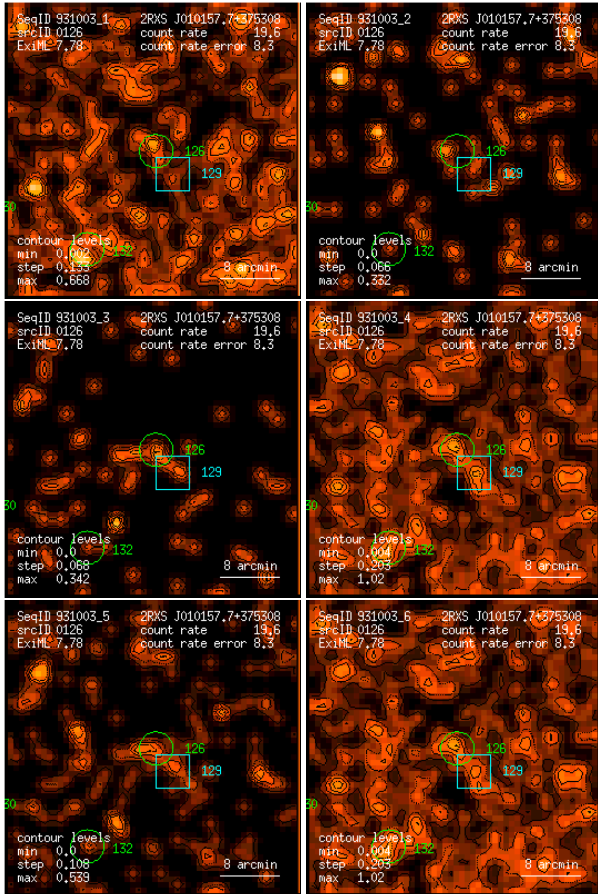
Figure 126: RASS 931003: detection 0126: band rate images, Gaussian filter: (1) PSPC channels 11 – 41, (2) 52 – 90, (3) 91 – 201, (4) 11 – 235, (5) 52 – 201, (6) 11 – 201. Broad band rates in counts/ks. Band rate contour levels in counts/ks/arcmin 2 .
