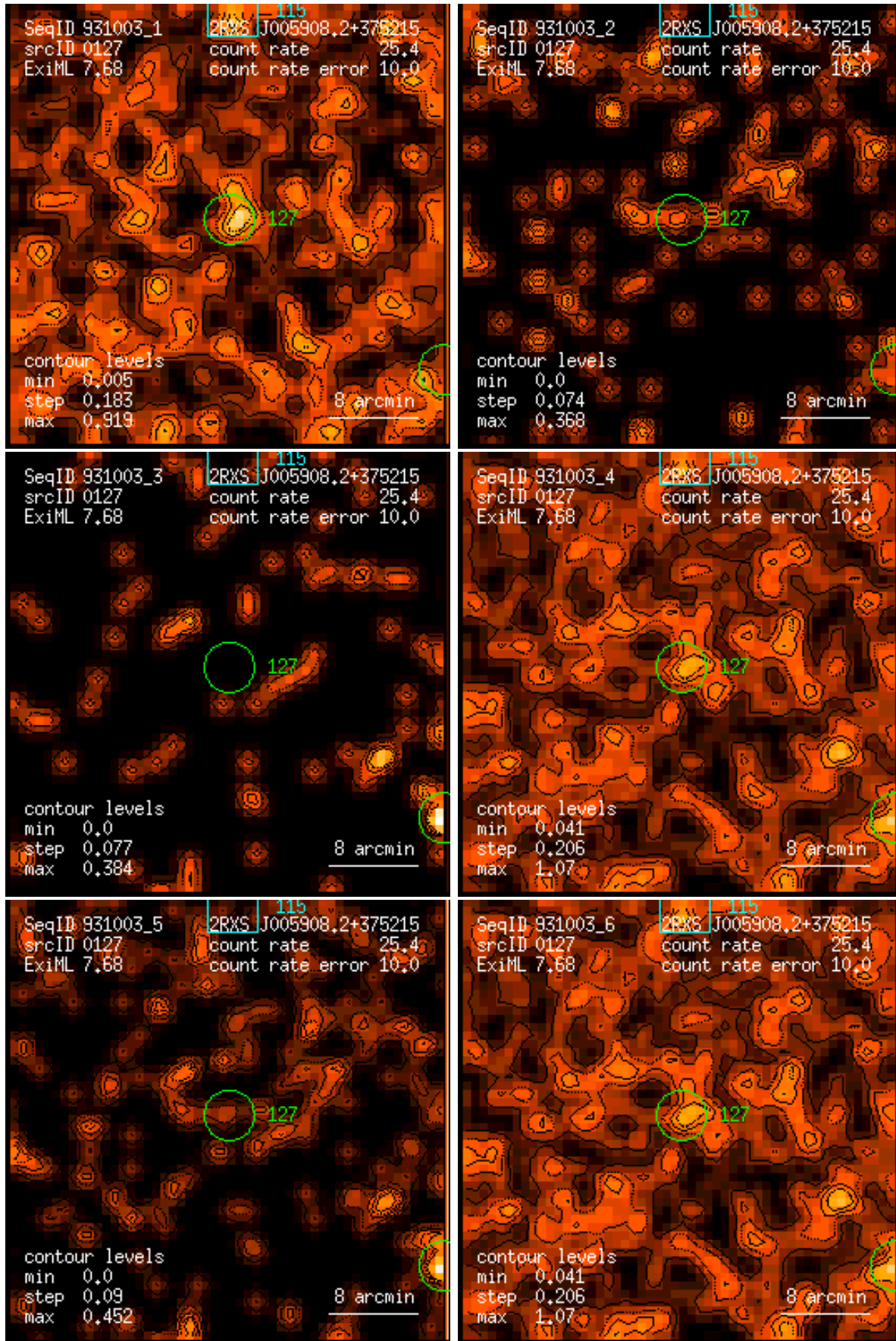
Figure 127: RASS 931003: detection 0127: band rate images, Gaussian filter: (1) PSPC channels 11 – 41, (2) 52 – 90, (3) 91 – 201, (4) 11 – 235, (5) 52 – 201, (6) 11 – 201. Broad band rates in counts/ks. Band rate contour levels in counts/ks/arcmin 2 .
