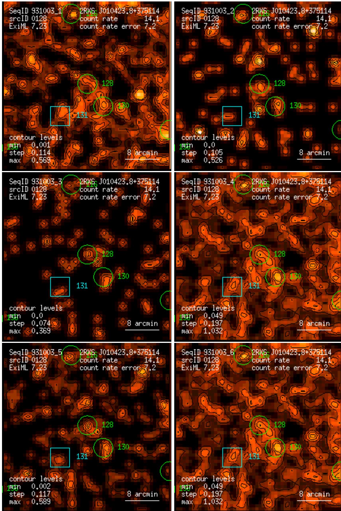
Figure 128: RASS 931003: detection 0128: band rate images, Gaussian filter: (1) PSPC channels 11 – 41, (2) 52 – 90, (3) 91 – 201, (4) 11 – 235, (5) 52 – 201, (6) 11 – 201. Broad band rates in counts/ks. Band rate contour levels in counts/ks/arcmin 2 .
