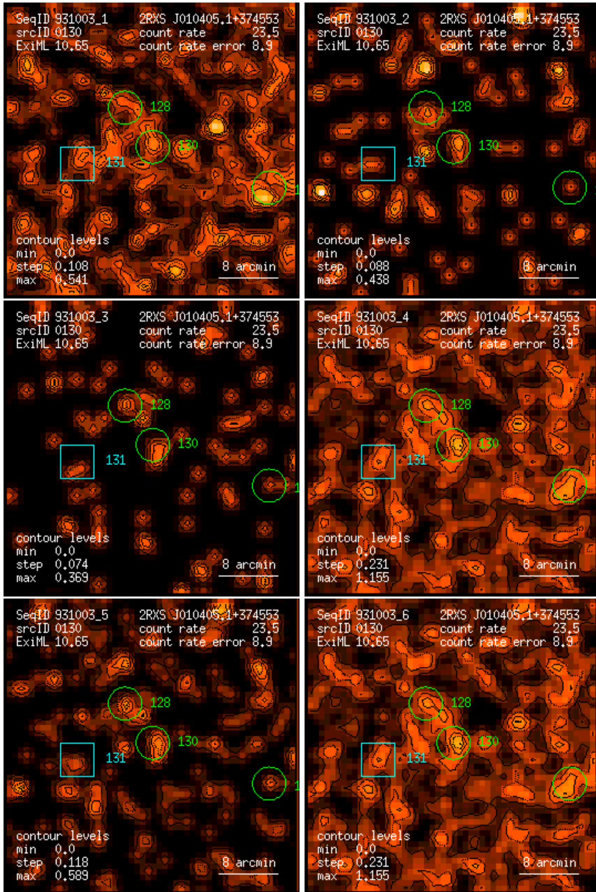
Figure 130: RASS 931003: detection 0130: band rate images, Gaussian filter: (1) PSPC channels 11 – 41, (2) 52 – 90, (3) 91 – 201, (4) 11 – 235, (5) 52 – 201, (6) 11 – 201. Broad band rates in counts/ks. Band rate contour levels in counts/ks/arcmin 2 .
