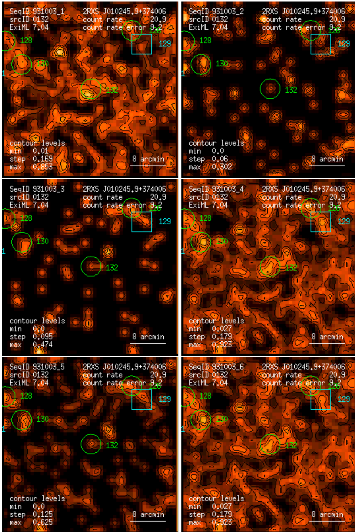
Figure 132: RASS 931003: detection 0132: band rate images, Gaussian filter: (1) PSPC channels 11 – 41, (2) 52 – 90, (3) 91 – 201, (4) 11 – 235, (5) 52 – 201, (6) 11 – 201. Broad band rates in counts/ks. Band rate contour levels in counts/ks/arcmin 2 .
