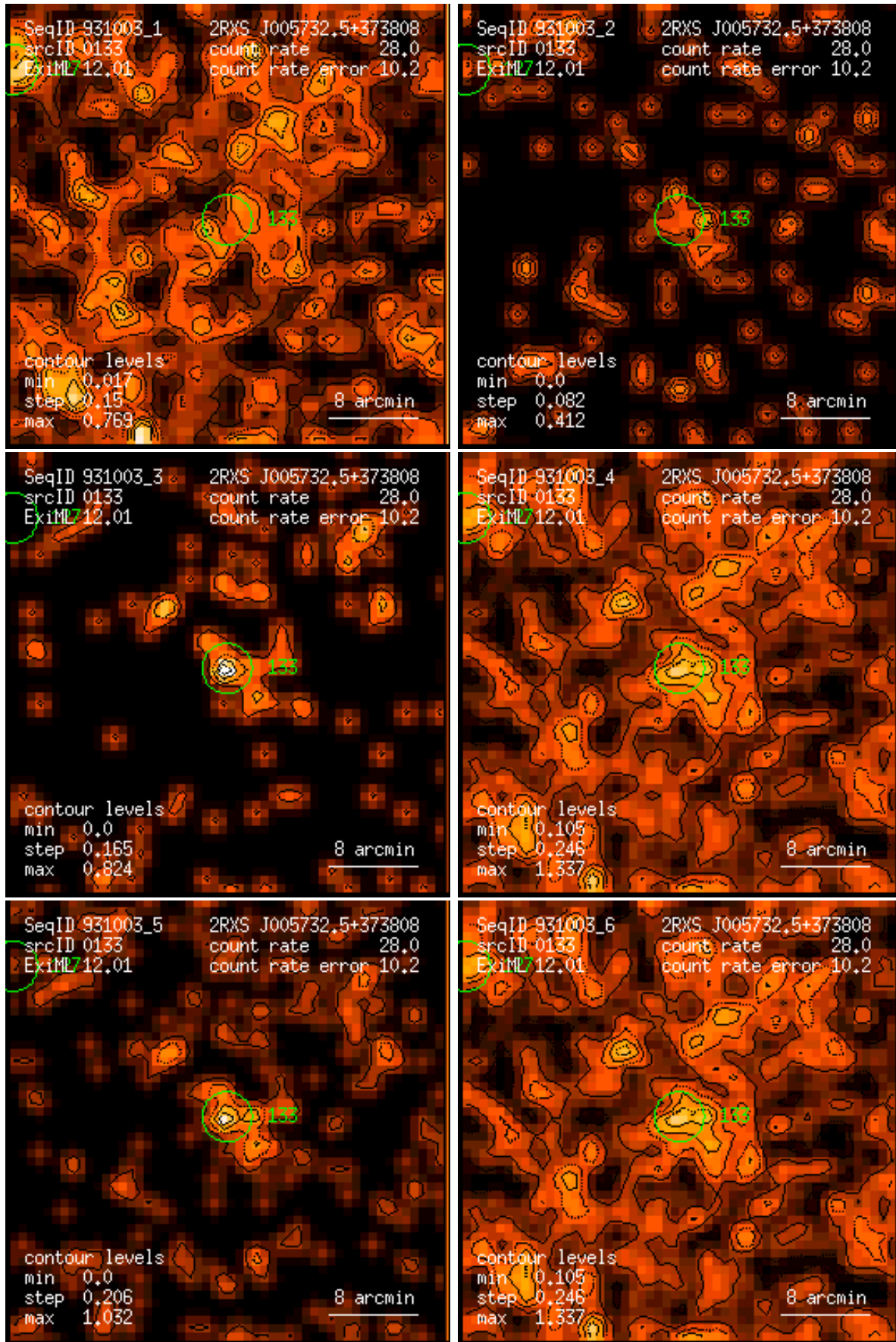
Figure 133: RASS 931003: detection 0133: band rate images, Gaussian filter: (1) PSPC channels 11 – 41, (2) 52 – 90, (3) 91 – 201, (4) 11 – 235, (5) 52 – 201, (6) 11 – 201. Broad band rates in counts/ks. Band rate contour levels in counts/ks/arcmin 2 .
