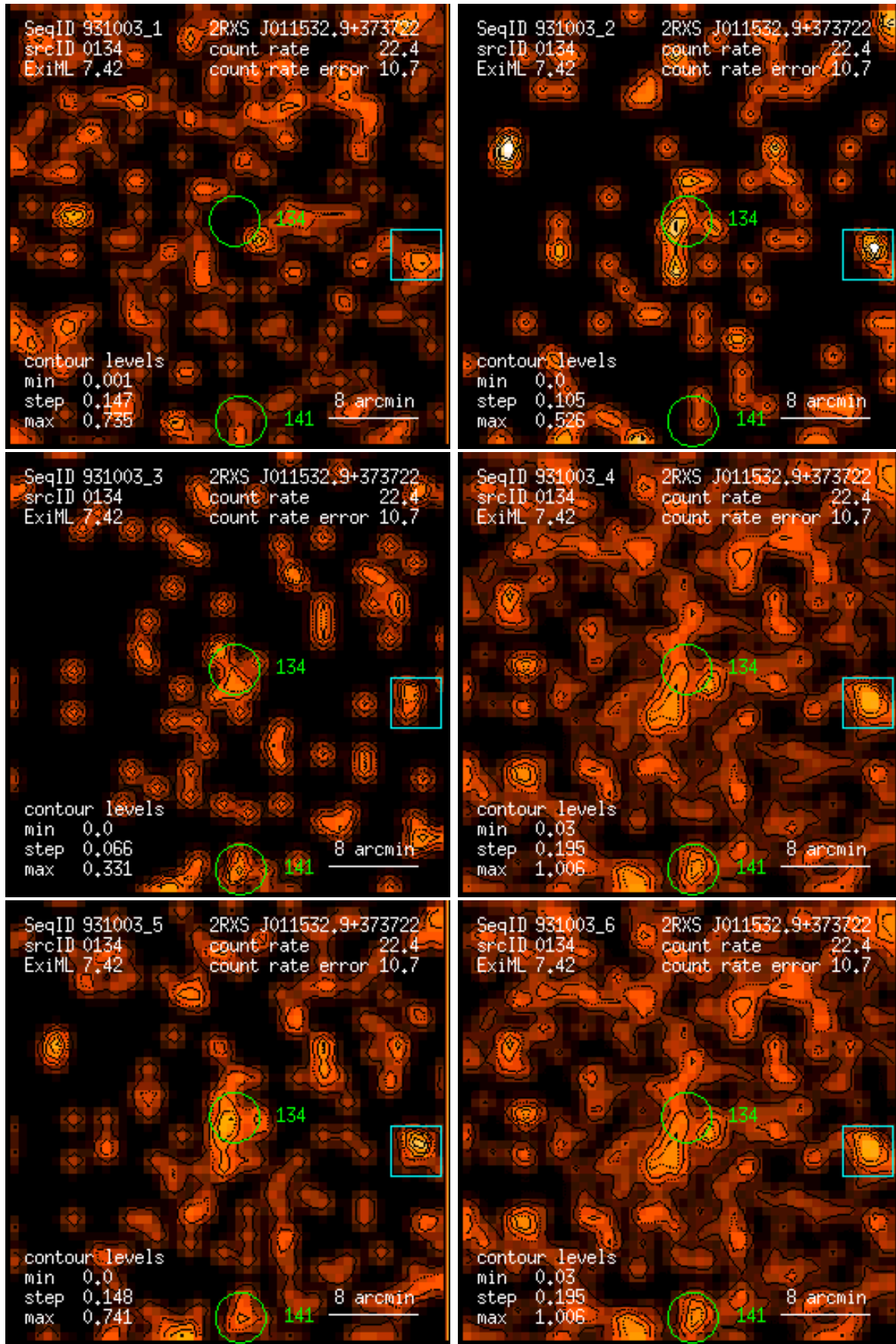
Figure 134: RASS 931003: detection 0134: band rate images, Gaussian filter: (1) PSPC channels 11 – 41, (2) 52 – 90, (3) 91 – 201, (4) 11 – 235, (5) 52 – 201, (6) 11 – 201. Broad band rates in counts/ks. Band rate contour levels in counts/ks/arcmin 2 .
