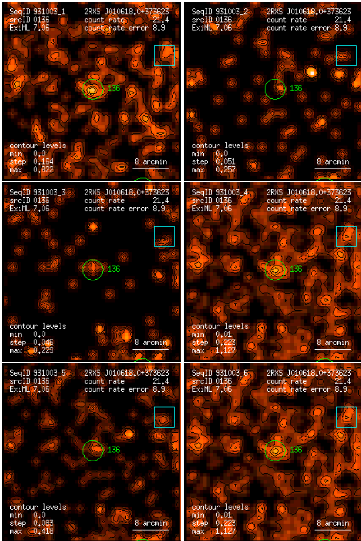
Figure 136: RASS 931003: detection 0136: band rate images, Gaussian filter: (1) PSPC channels 11 – 41, (2) 52 – 90, (3) 91 – 201, (4) 11 – 235, (5) 52 – 201, (6) 11 – 201. Broad band rates in counts/ks. Band rate contour levels in counts/ks/arcmin 2 .
