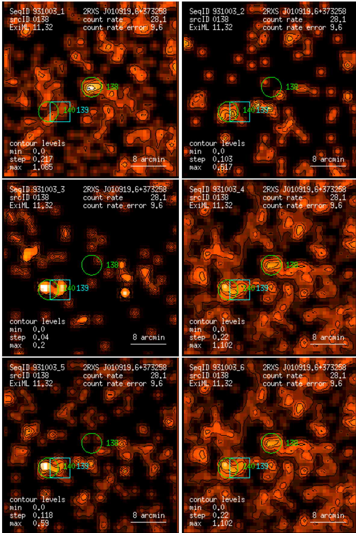
Figure 138: RASS 931003: detection 0138: band rate images, Gaussian filter: (1) PSPC channels 11 – 41, (2) 52 – 90, (3) 91 – 201, (4) 11 – 235, (5) 52 – 201, (6) 11 – 201. Broad band rates in counts/ks. Band rate contour levels in counts/ks/arcmin 2 .
