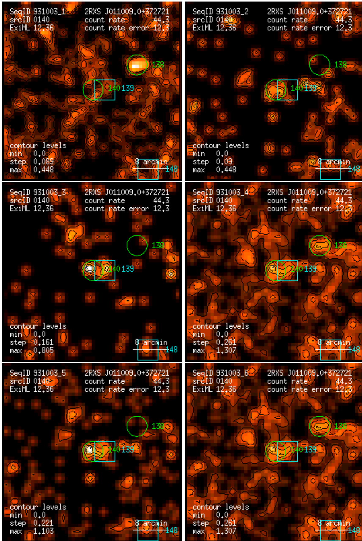
Figure 140: RASS 931003: detection 0140: band rate images, Gaussian filter: (1) PSPC channels 11 – 41, (2) 52 – 90, (3) 91 – 201, (4) 11 – 235, (5) 52 – 201, (6) 11 – 201. Broad band rates in counts/ks. Band rate contour levels in counts/ks/arcmin 2 .
