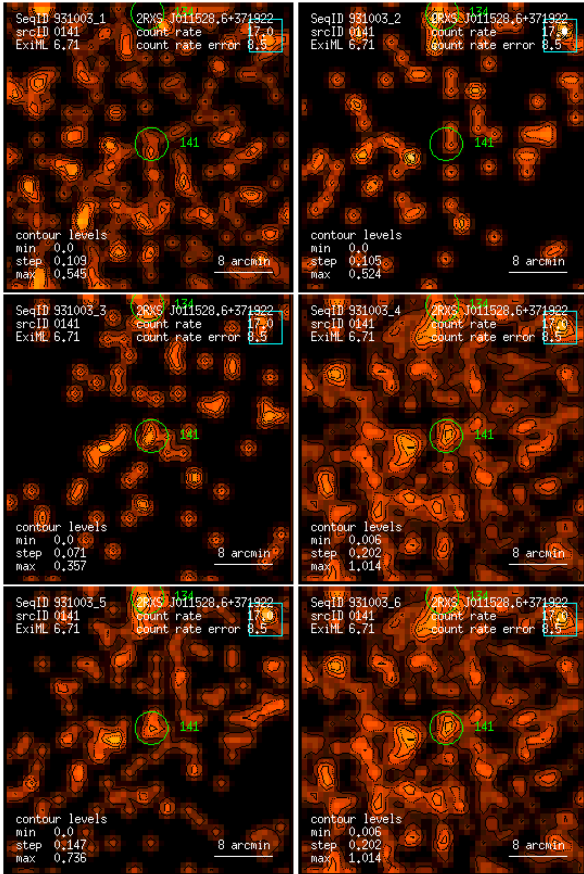
Figure 141: RASS 931003: detection 0141: band rate images, Gaussian filter: (1) PSPC channels 11 – 41, (2) 52 – 90, (3) 91 – 201, (4) 11 – 235, (5) 52 – 201, (6) 11 – 201. Broad band rates in counts/ks. Band rate contour levels in counts/ks/arcmin 2 .
