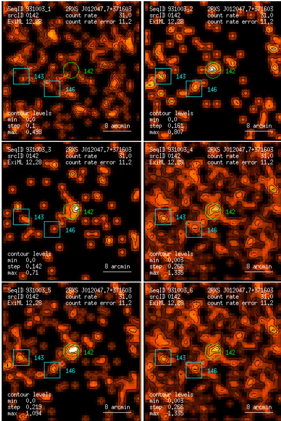
Figure 142: RASS 931003: detection 0142: band rate images, Gaussian filter: (1) PSPC channels 11 – 41, (2) 52 – 90, (3) 91 – 201, (4) 11 – 235, (5) 52 – 201, (6) 11 – 201. Broad band rates in counts/ks. Band rate contour levels in counts/ks/arcmin 2 .
