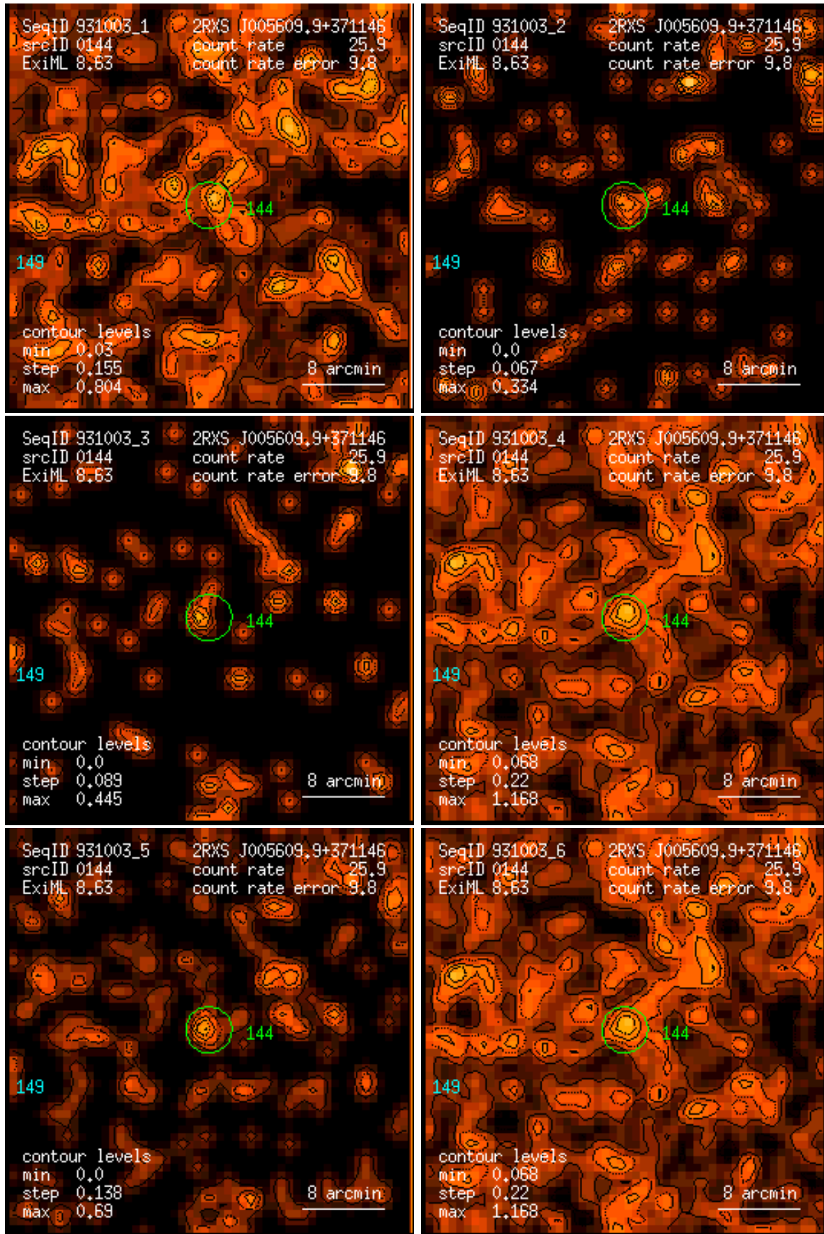
Figure 144: RASS 931003: detection 0144: band rate images, Gaussian filter: (1) PSPC channels 11 – 41, (2) 52 – 90, (3) 91 – 201, (4) 11 – 235, (5) 52 – 201, (6) 11 – 201. Broad band rates in counts/ks. Band rate contour levels in counts/ks/arcmin 2 .
