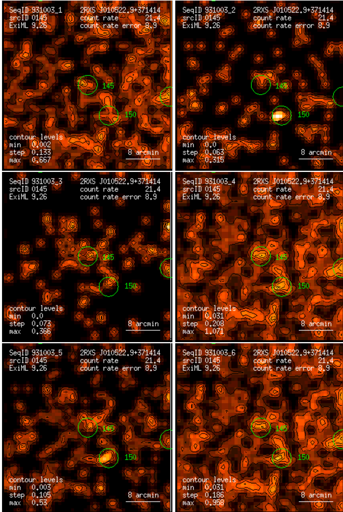
Figure 145: RASS 931003: detection 0145: band rate images, Gaussian filter: (1) PSPC channels 11 – 41, (2) 52 – 90, (3) 91 – 201, (4) 11 – 235, (5) 52 – 201, (6) 11 – 201. Broad band rates in counts/ks. Band rate contour levels in counts/ks/arcmin 2 .
