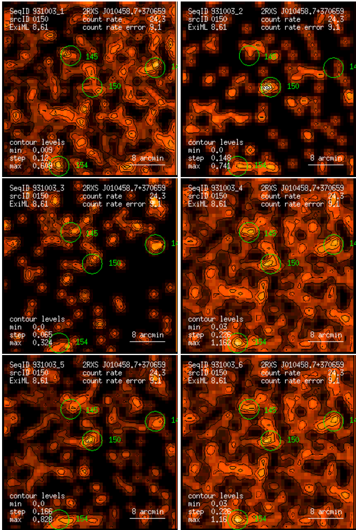
Figure 150: RASS 931003: detection 0150: band rate images, Gaussian filter: (1) PSPC channels 11 – 41, (2) 52 – 90, (3) 91 – 201, (4) 11 – 235, (5) 52 – 201, (6) 11 – 201. Broad band rates in counts/ks. Band rate contour levels in counts/ks/arcmin 2 .
