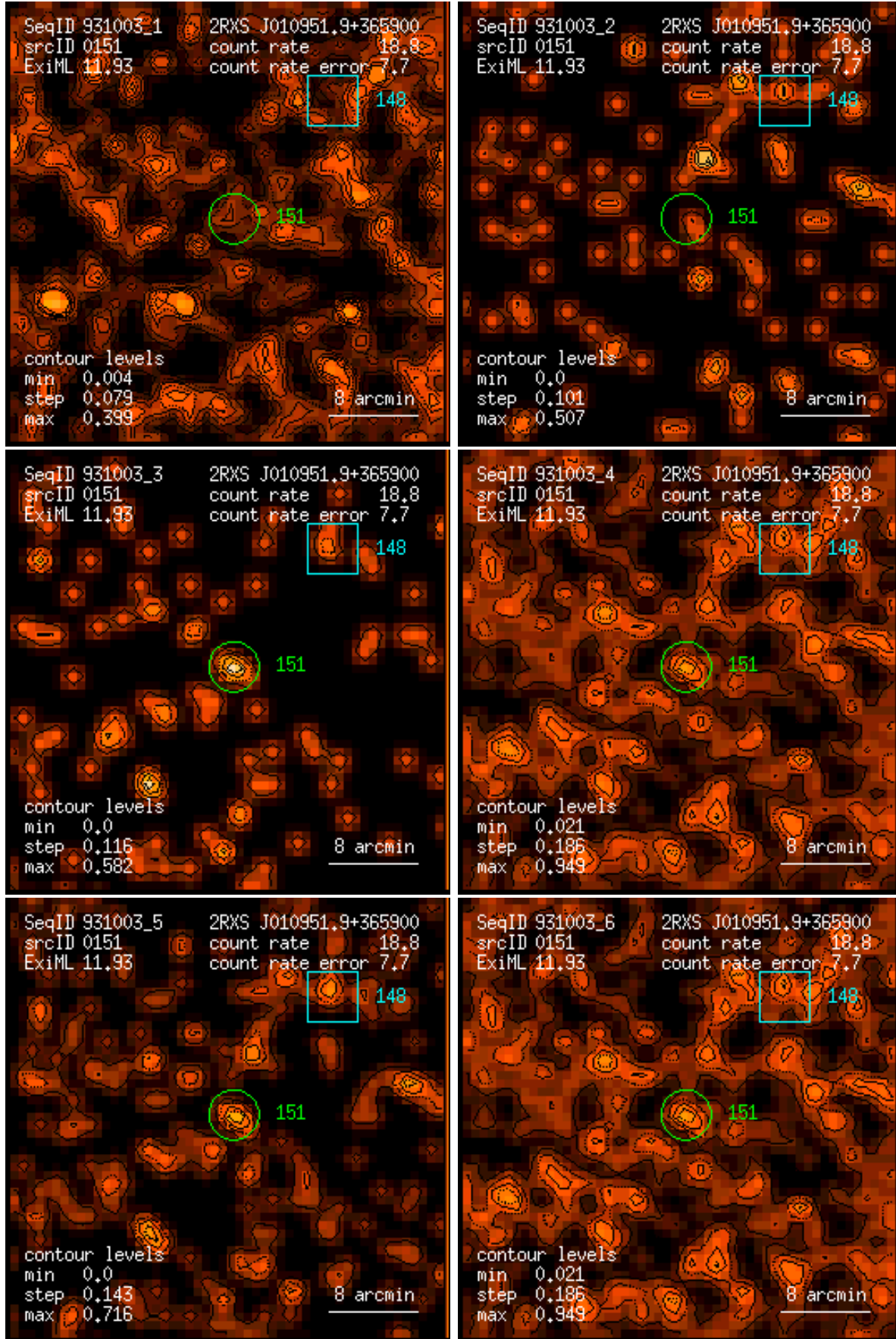
Figure 151: RASS 931003: detection 0151: band rate images, Gaussian filter: (1) PSPC channels 11 – 41, (2) 52 – 90, (3) 91 – 201, (4) 11 – 235, (5) 52 – 201, (6) 11 – 201. Broad band rates in counts/ks. Band rate contour levels in counts/ks/arcmin 2 .
