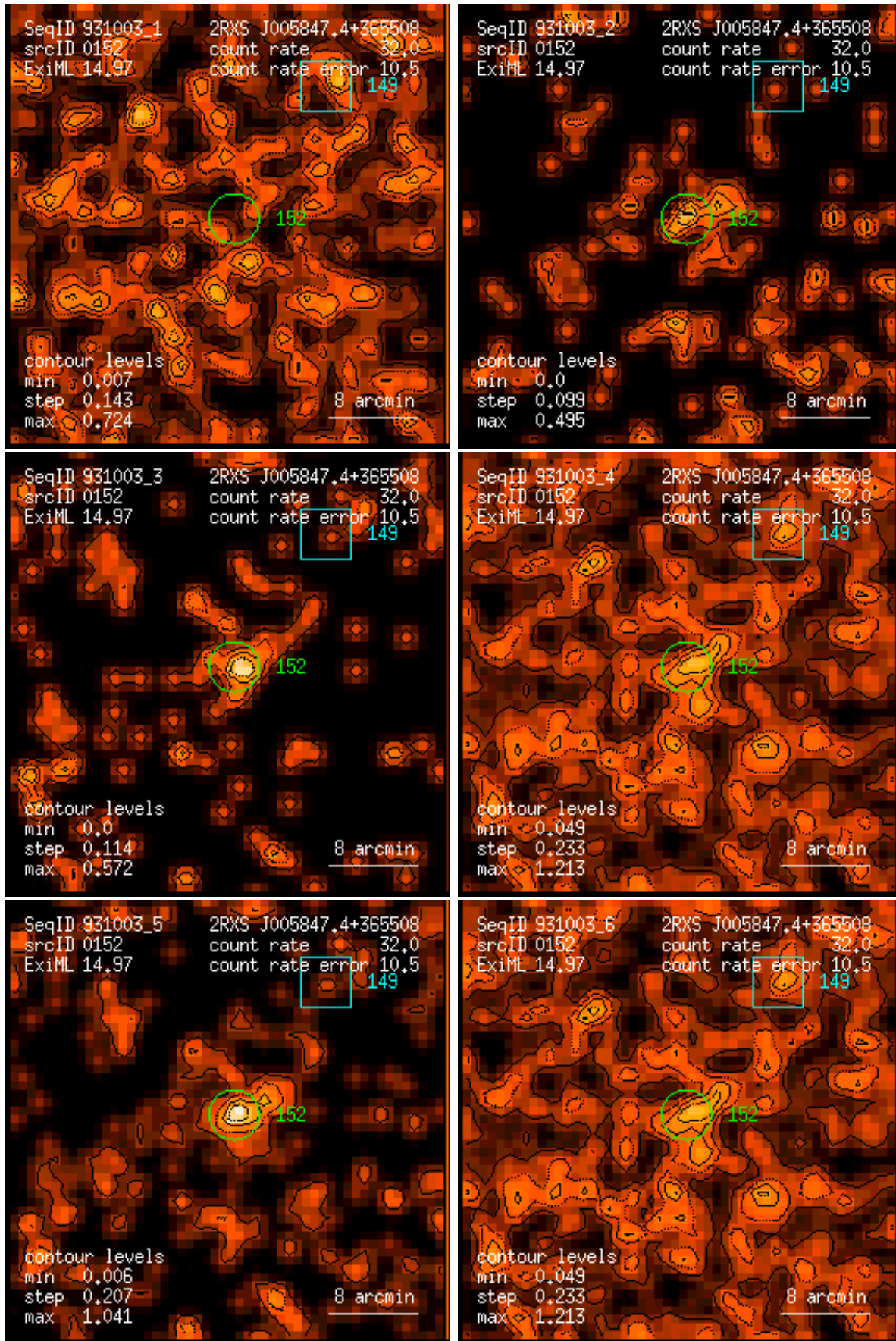
Figure 152: RASS 931003: detection 0152: band rate images, Gaussian filter: (1) PSPC channels 11 – 41, (2) 52 – 90, (3) 91 – 201, (4) 11 – 235, (5) 52 – 201, (6) 11 – 201. Broad band rates in counts/ks. Band rate contour levels in counts/ks/arcmin 2 .
