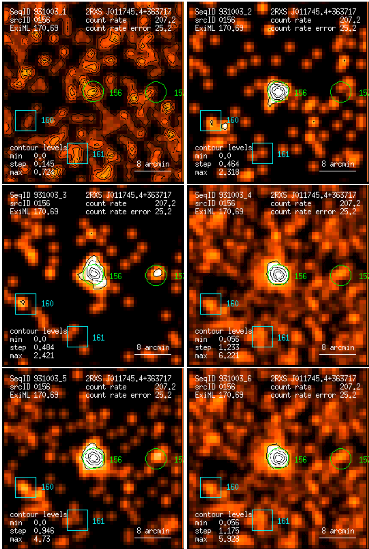
Figure 156: RASS 931003: detection 0156: band rate images, Gaussian filter: (1) PSPC channels 11 – 41, (2) 52 – 90, (3) 91 – 201, (4) 11 – 235, (5) 52 – 201, (6) 11 – 201. Broad band rates in counts/ks. Band rate contour levels in counts/ks/arcmin 2 .
