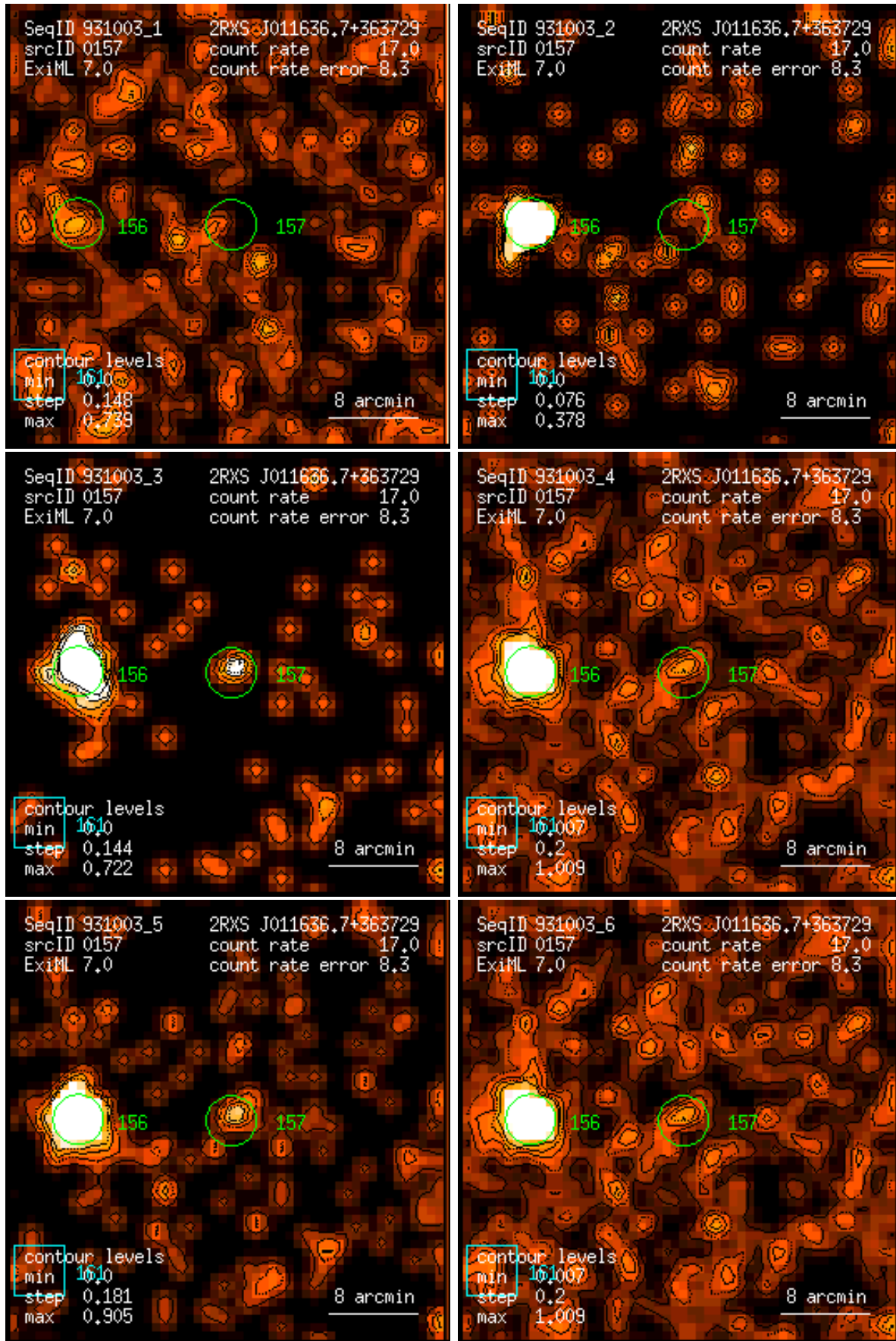
Figure 157: RASS 931003: detection 0157: band rate images, Gaussian filter: (1) PSPC channels 11 – 41, (2) 52 – 90, (3) 91 – 201, (4) 11 – 235, (5) 52 – 201, (6) 11 – 201. Broad band rates in counts/ks. Band rate contour levels in counts/ks/arcmin 2 .
